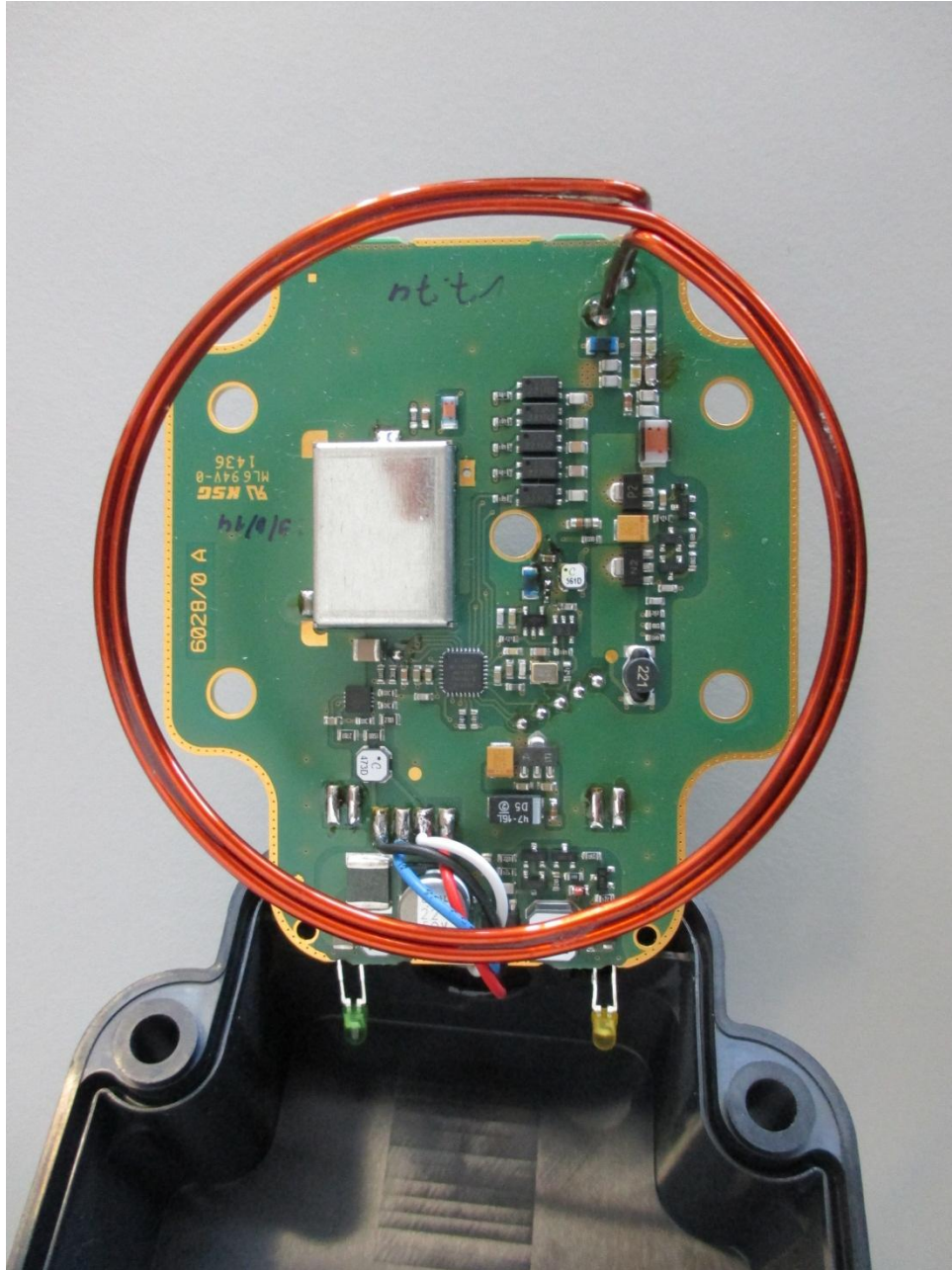
146178_9.JPG: TNSLR-Q80WD-H1147, PCB top view
