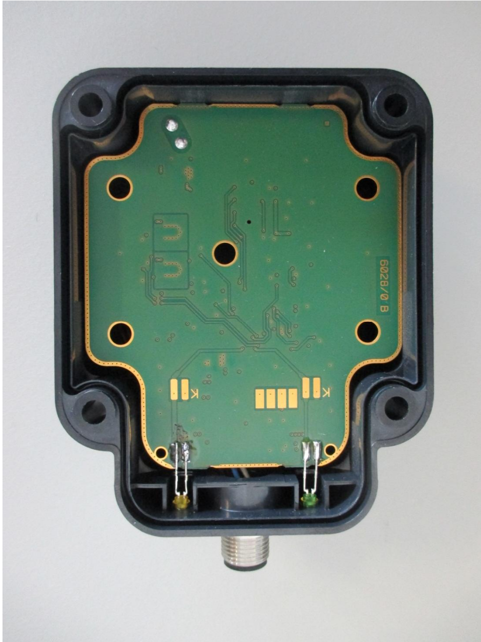
146178_10.JPG: TNSLR-Q80WD-H1147, PCB bottom view
