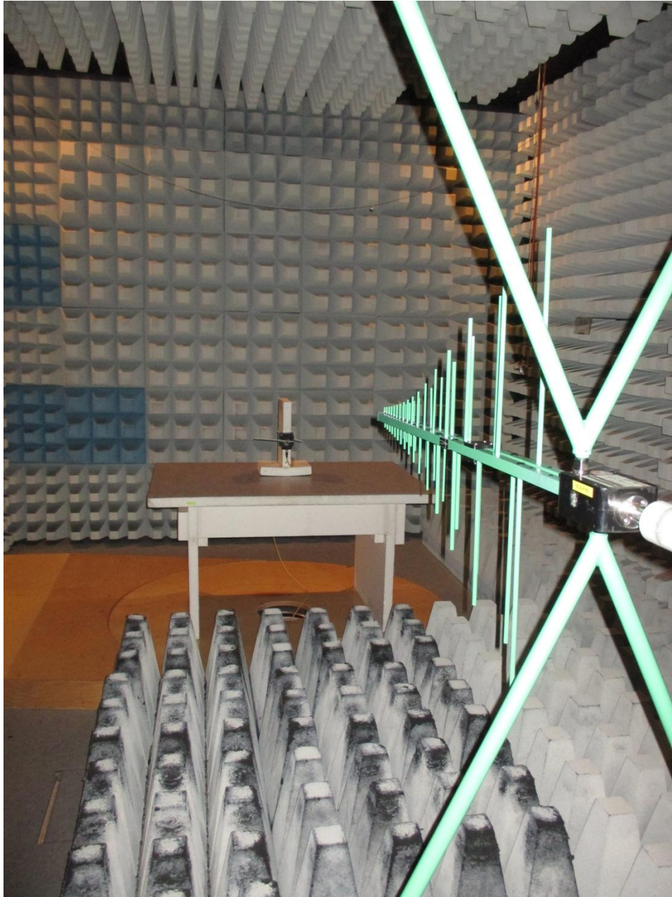
146178_2.JPG: Test setup fully anechoic chamber (E-Field)
