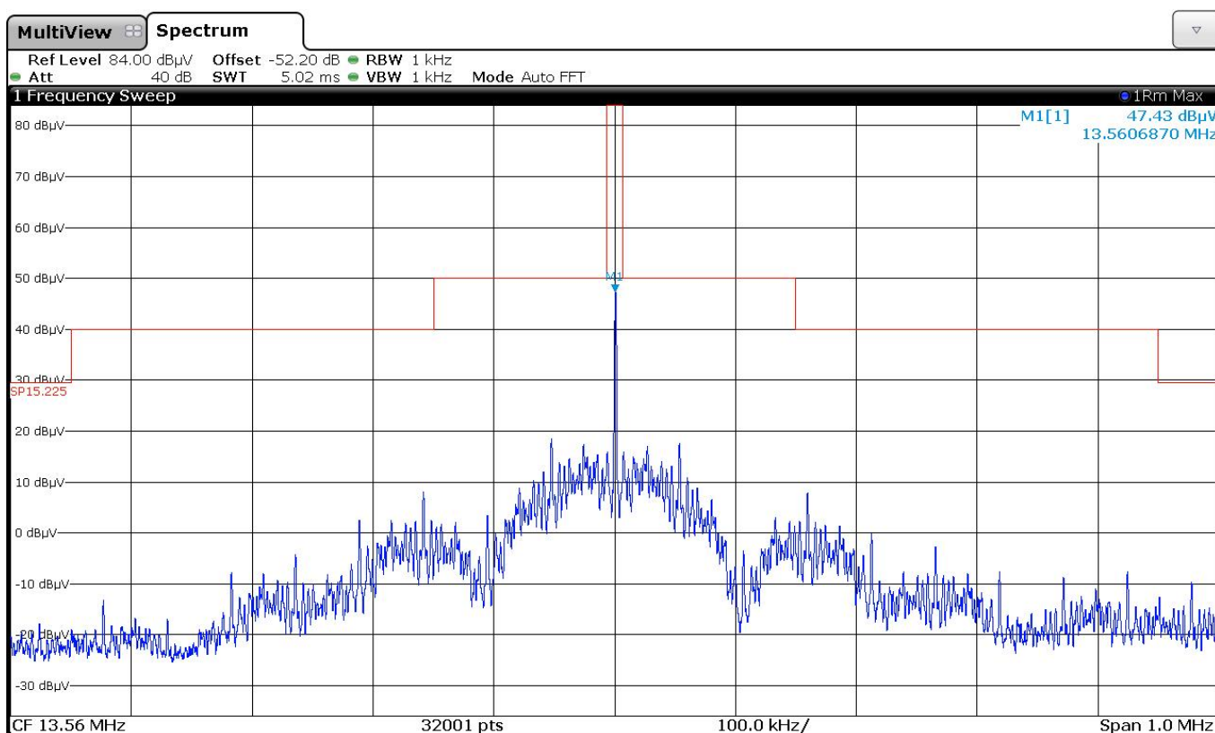
TNSLR-Q80WD-H1147_20deg_24V_FCC.png: Spectrum mask
