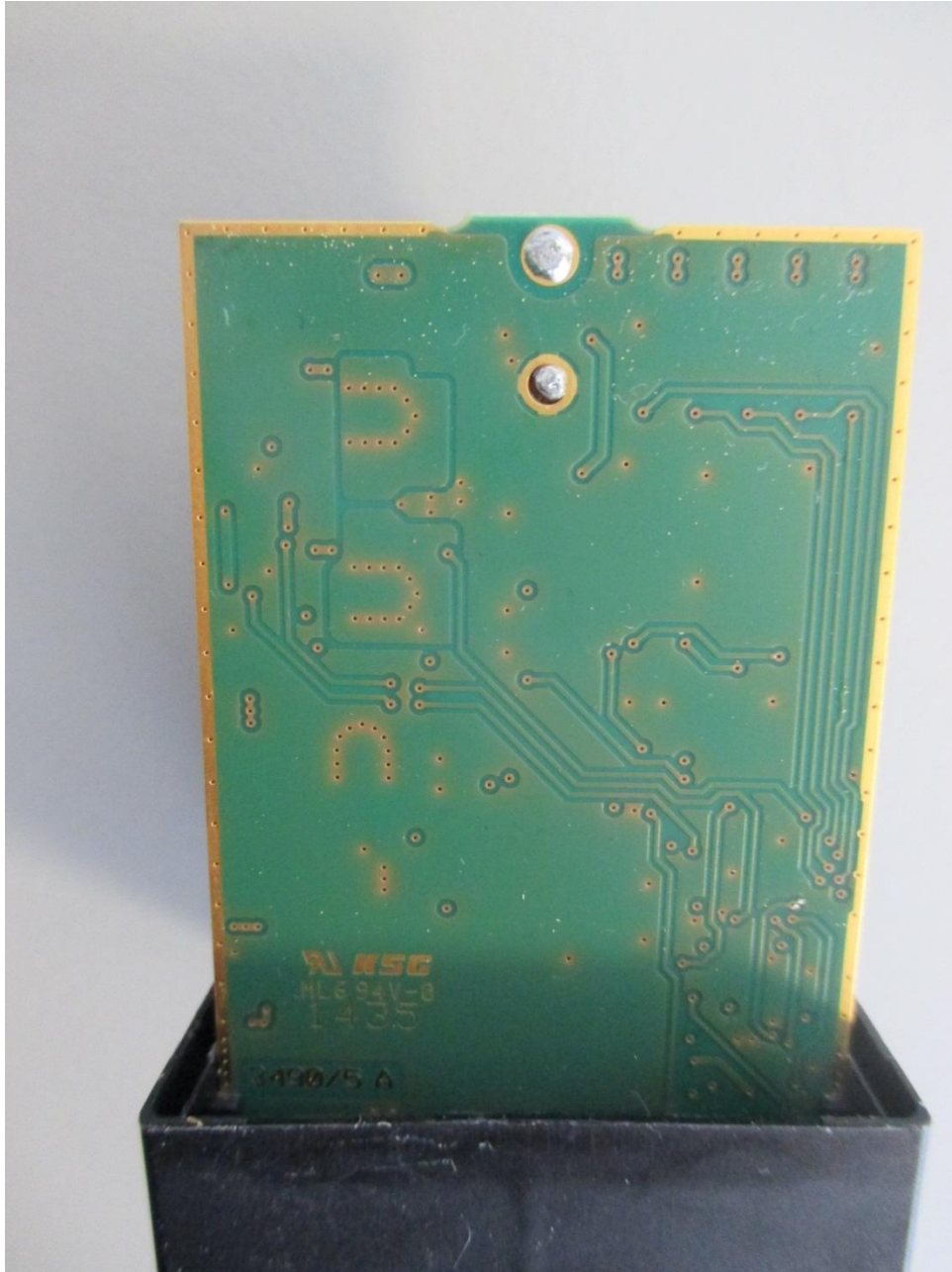
146179_10.JPG: TNSLR-Q42TWD-H1147, PCB bottom view
