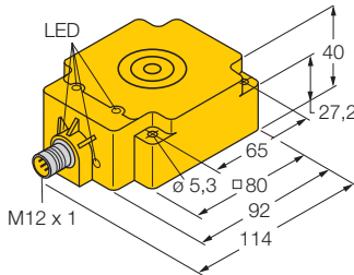
Figure 21 TN-Q80-H1147
