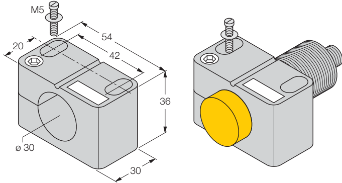
Figure 10 Mounting clip BST-30N
