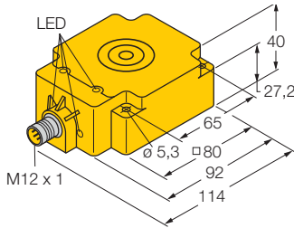
Figure 22 TN-Q80-H1147/ S1126
