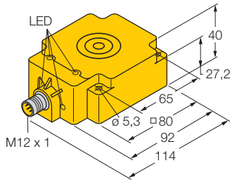
Figure 24 TNLR-Q80-H1147
