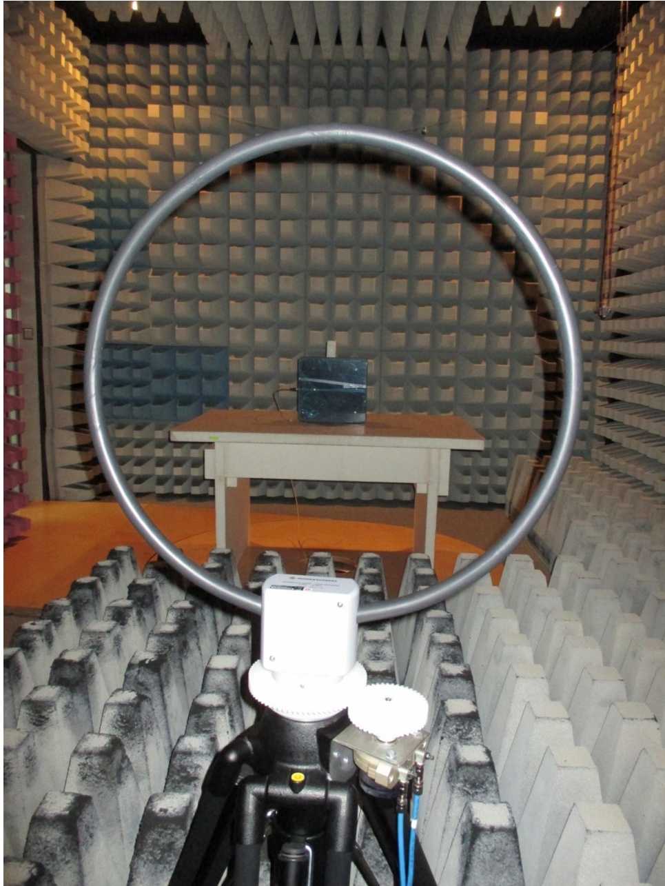
150243_3.JPG: Test setup fully anechoic chamber (H-Field)
