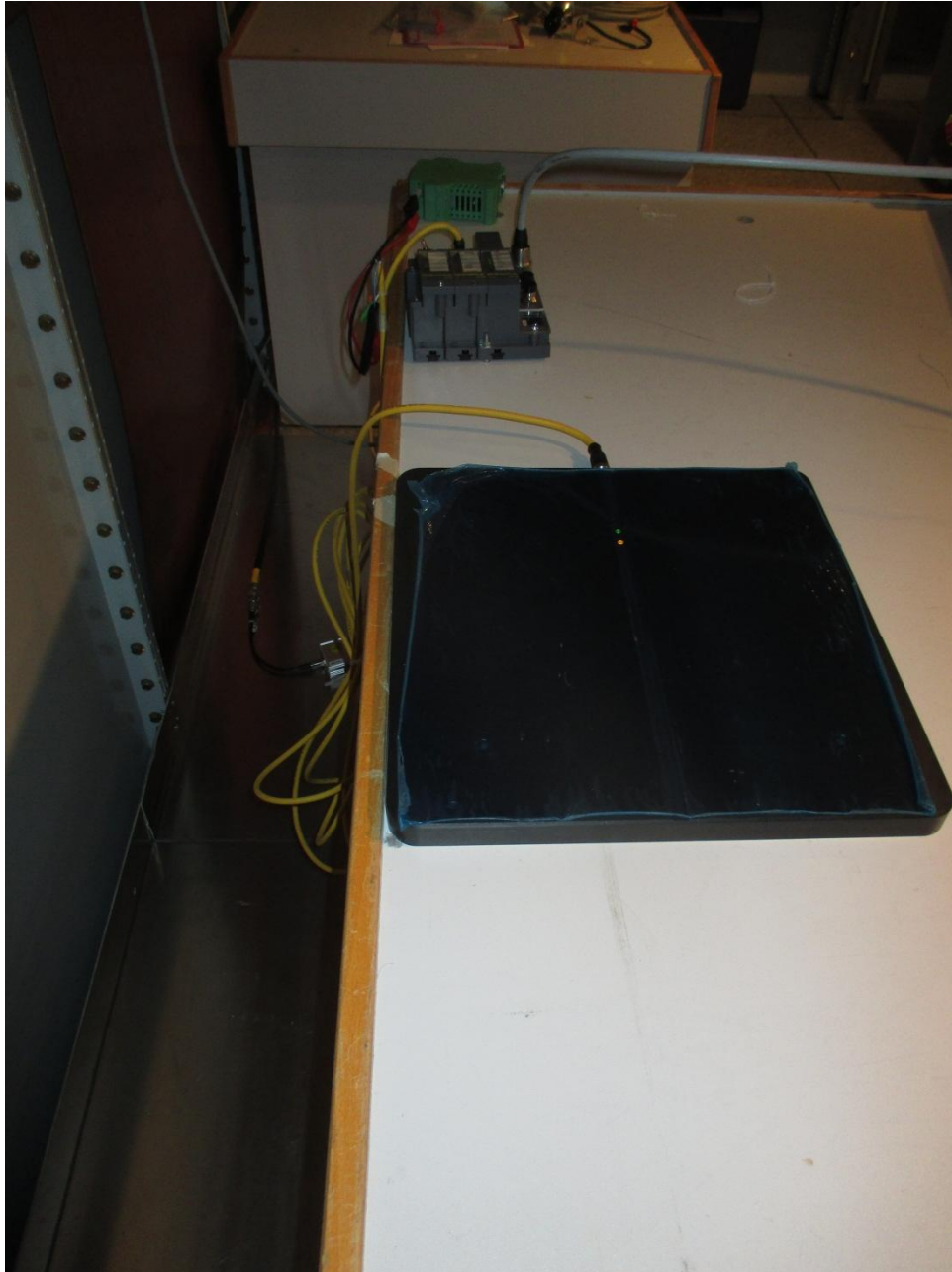
150243_1.JPG: Test setup shielded chamber
