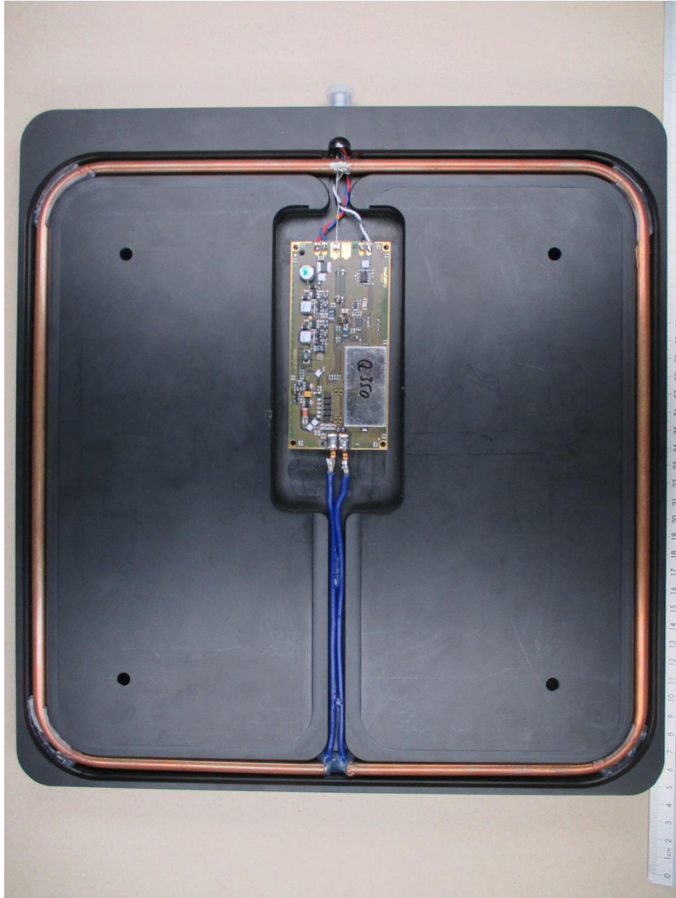
150243_10.JPG: TNSLR-Q350-H1147, bottom view
