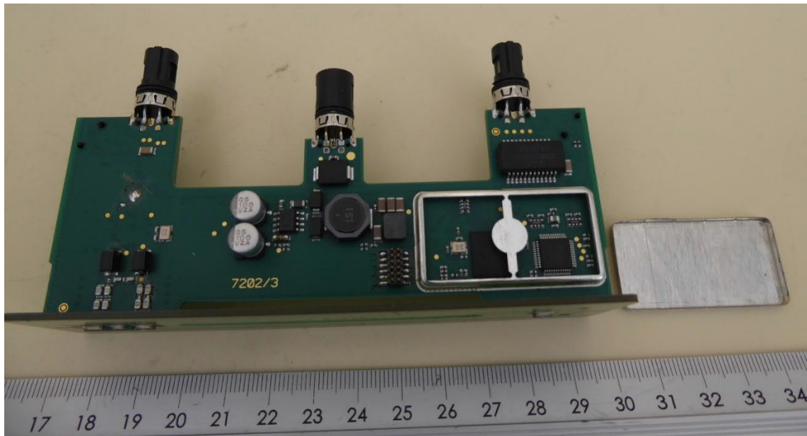
PCB view Top with opened shielding
