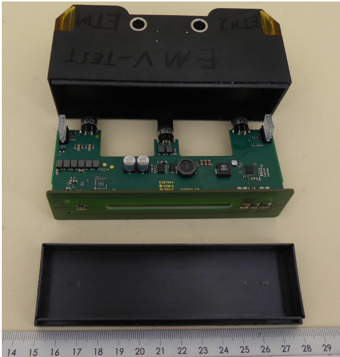
Internal view 2
