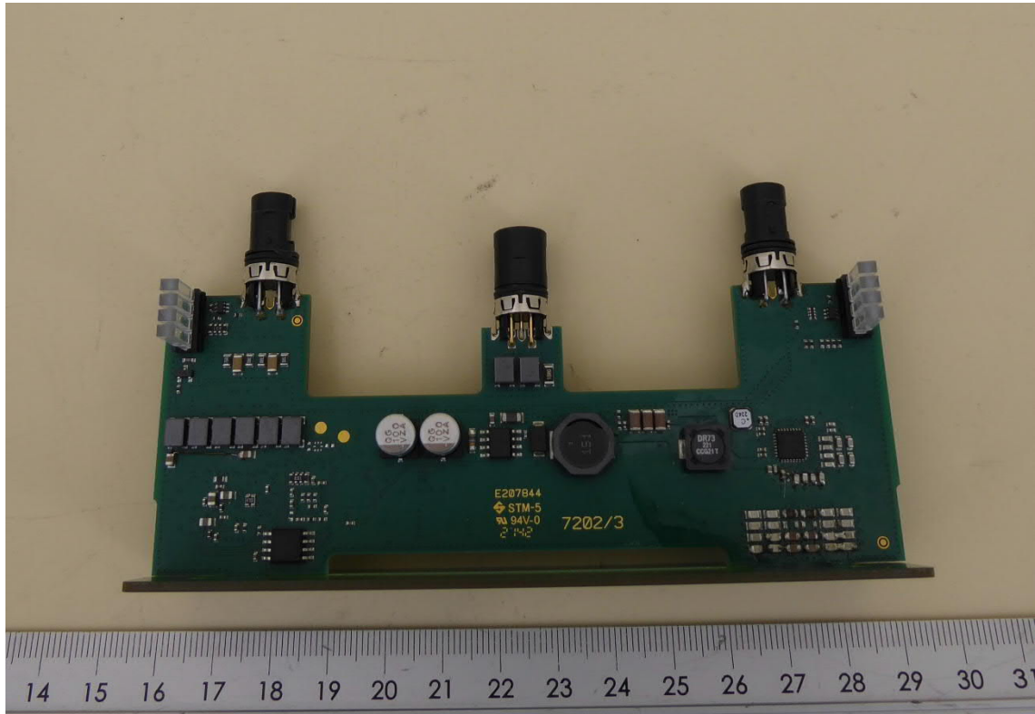
Internal view Bottom
