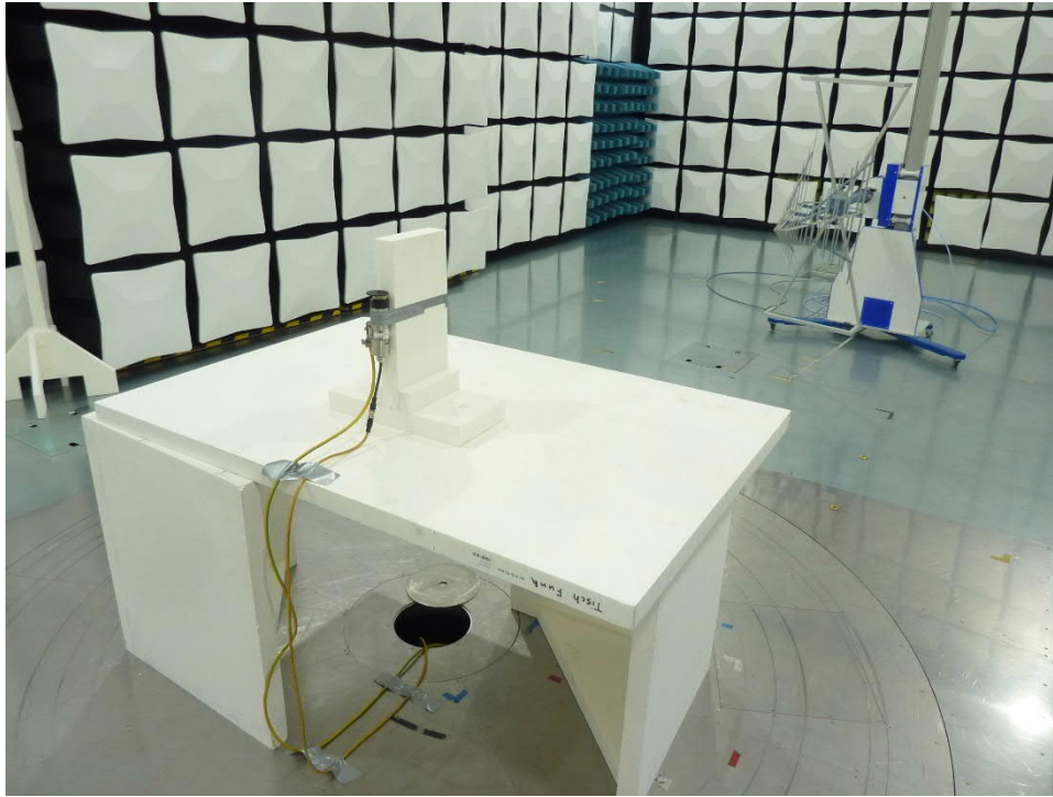
211147_07: Test setup preliminary measurement 30 MHz – 1 GHz
