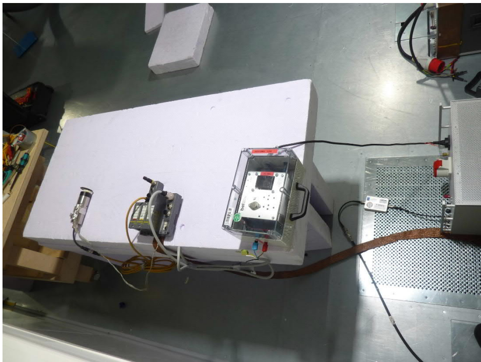
211147_02:Test setup conducted emission
