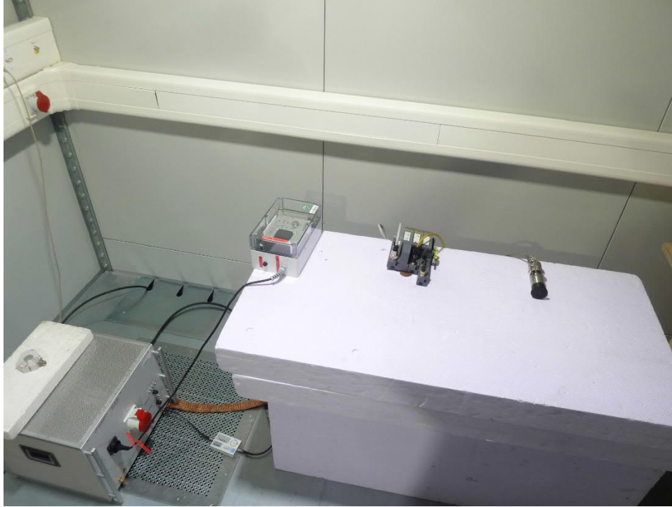
211147_01:Test setup conducted emission
