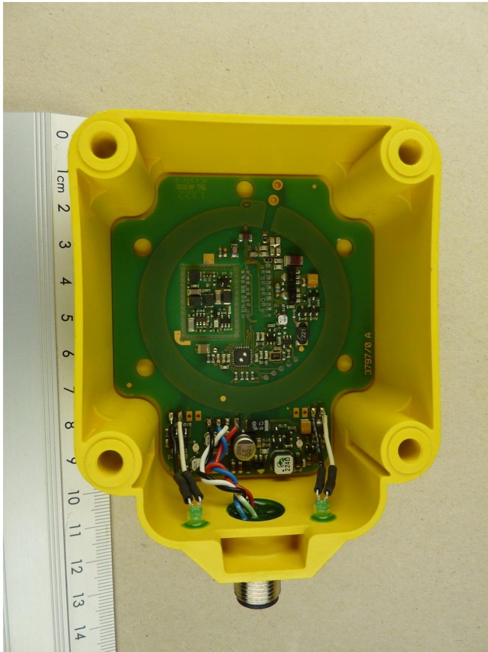
135058_6.JPG: TN-Q80-H1147, rear view to PCB
