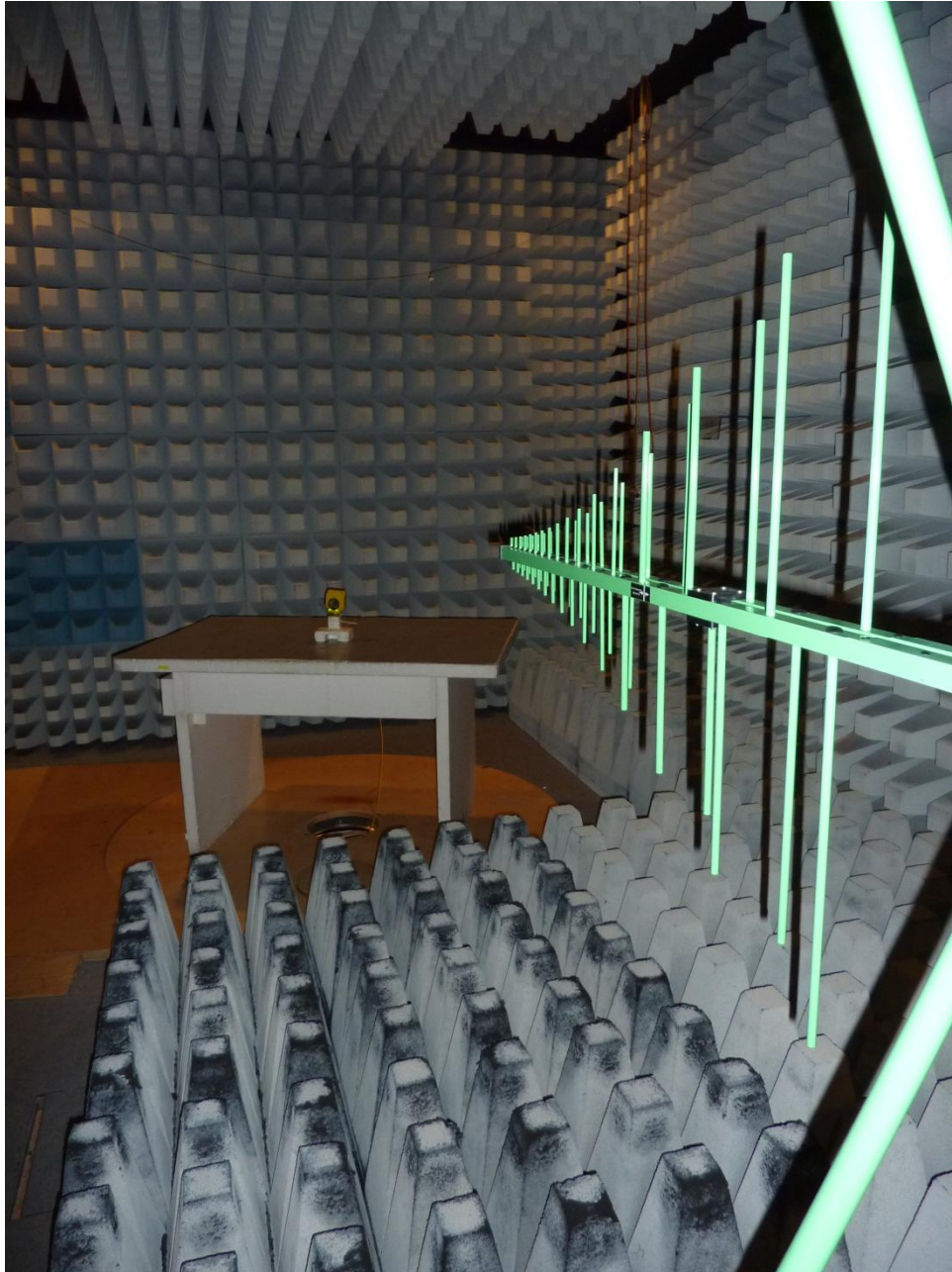
135058_11.JPG: Test setup fully anechoic chamber (E-Field)
