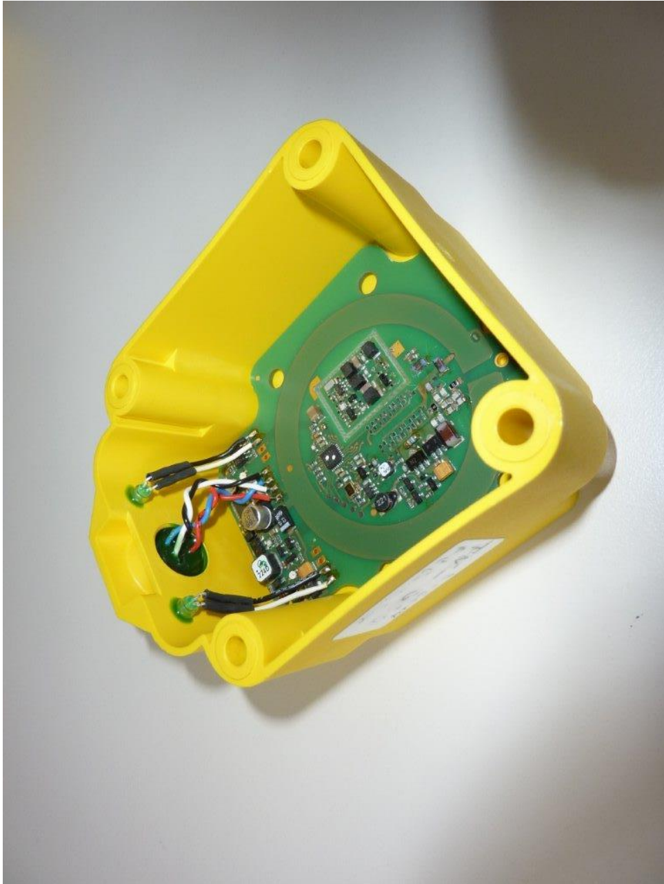
TN-Q80-H1147, 3D view 1
