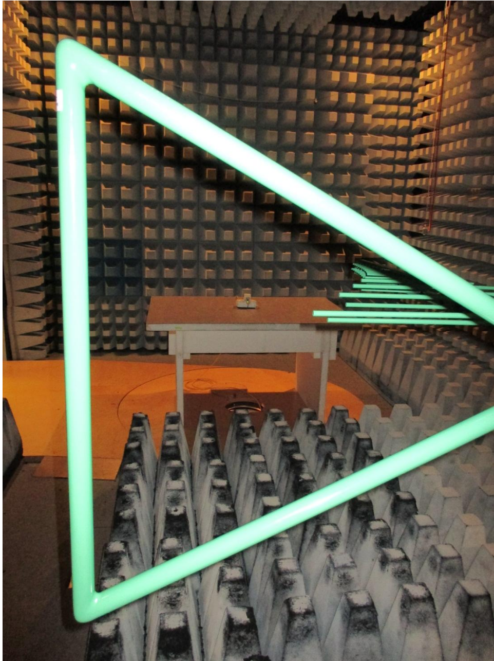
146168_2.JPG: Test setup fully anechoic chamber (E-Field)
