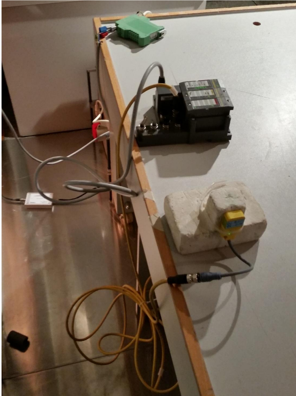
146168_1.jpg: Test setup shielded chamber
