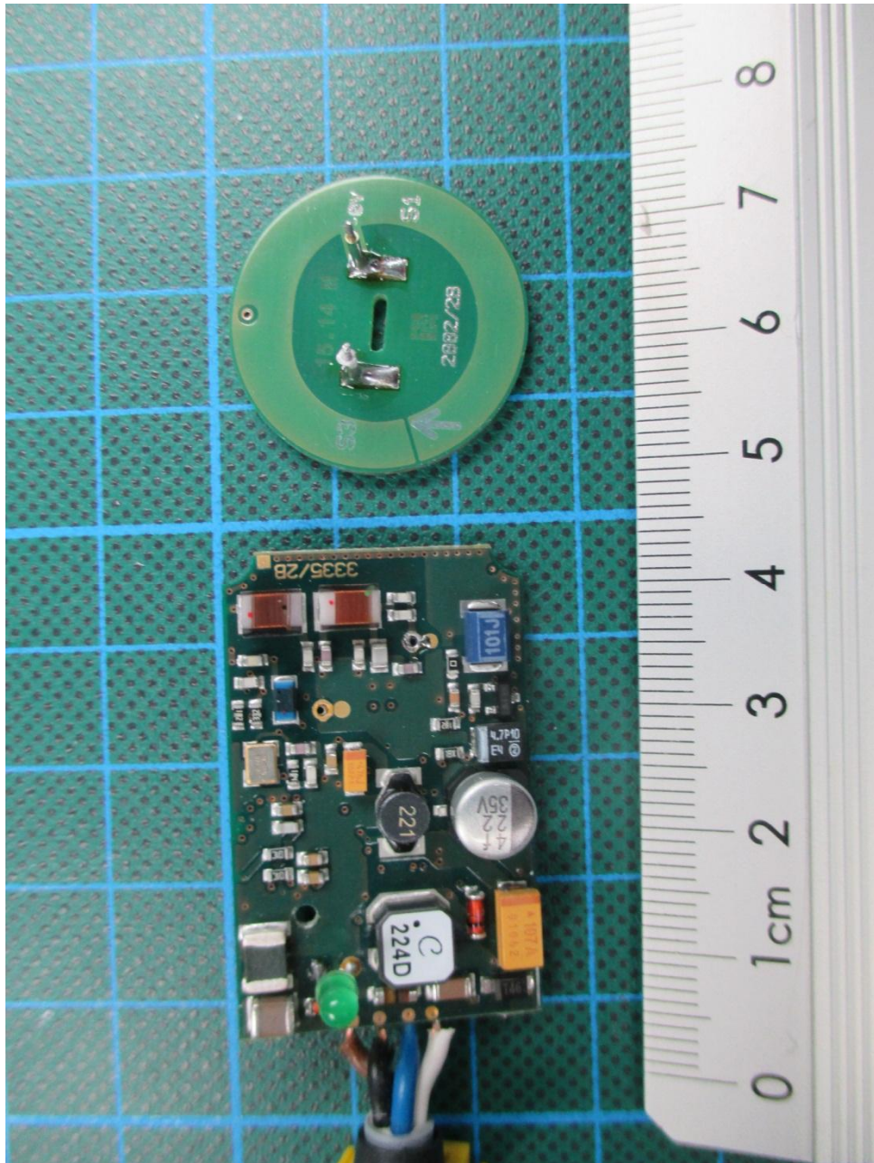
146168_14.JPG: TN-Q14-0.15-RS4.47T, PCB, front view antenna removed
