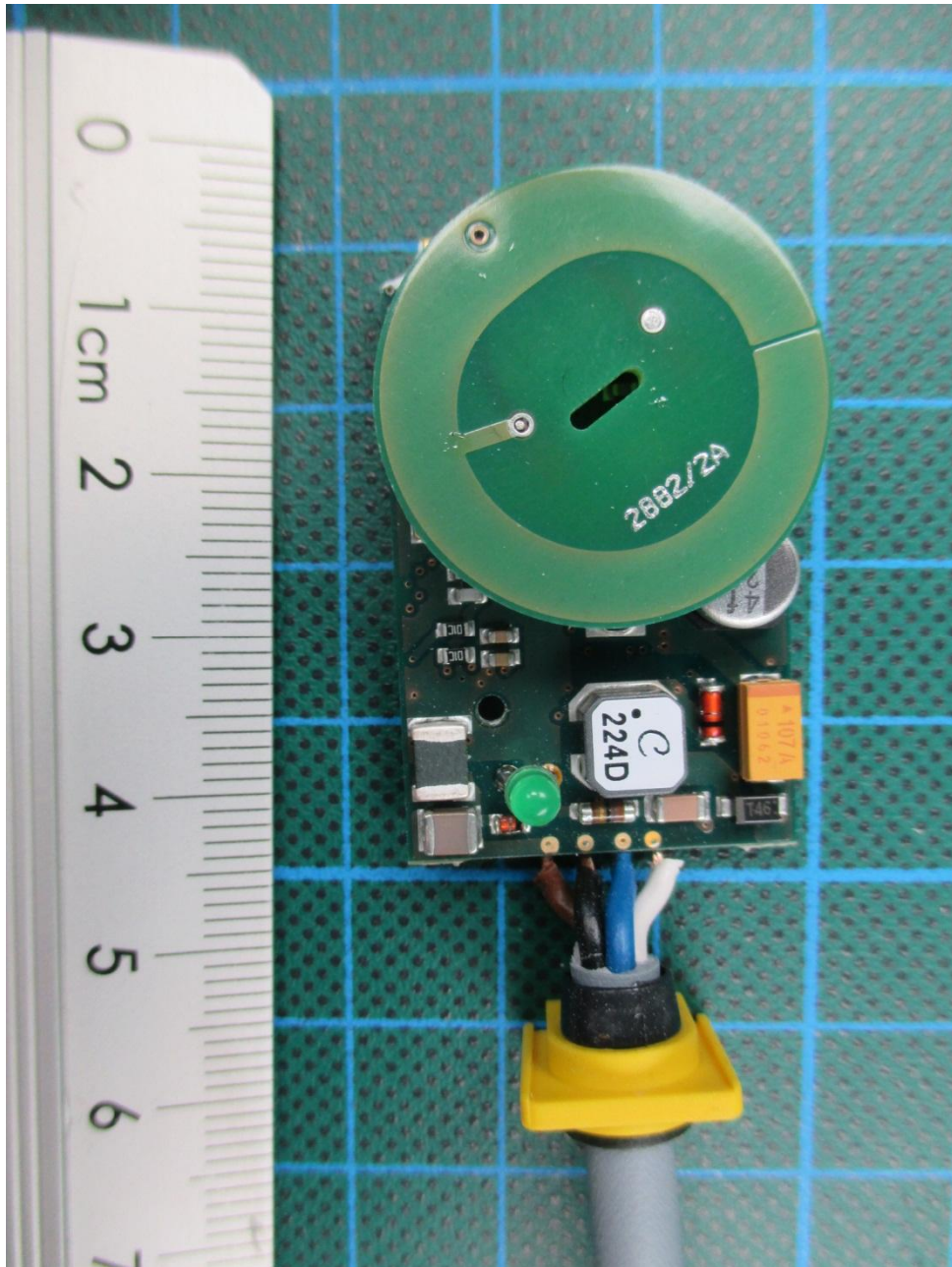
146168_13.JPG: TN-Q14-0.15-RS4.47T, PCB, front view with antenna
