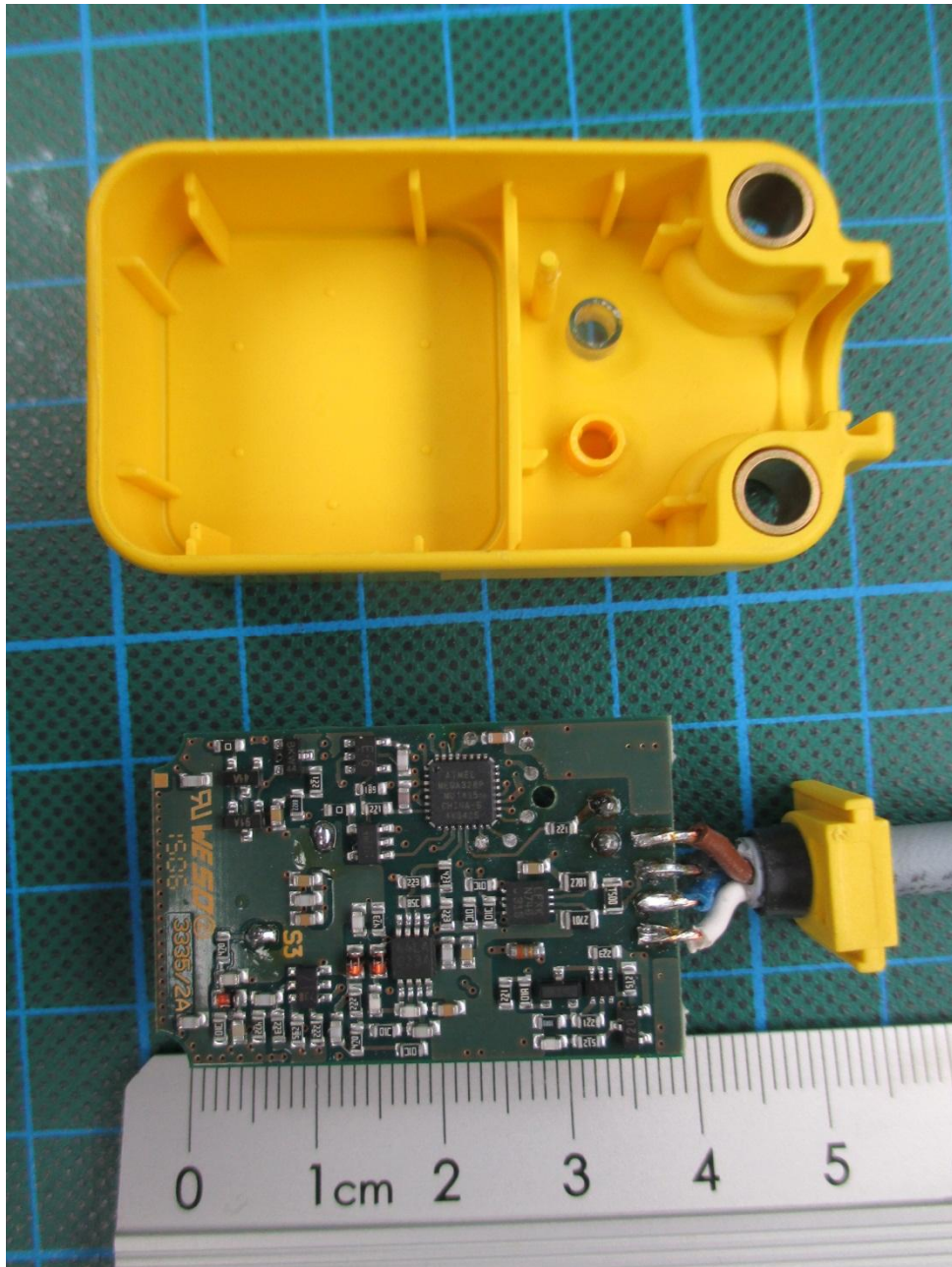
146168_11.JPG: TN-Q14-0.15-RS4.47T, PCB, rear view and housing
