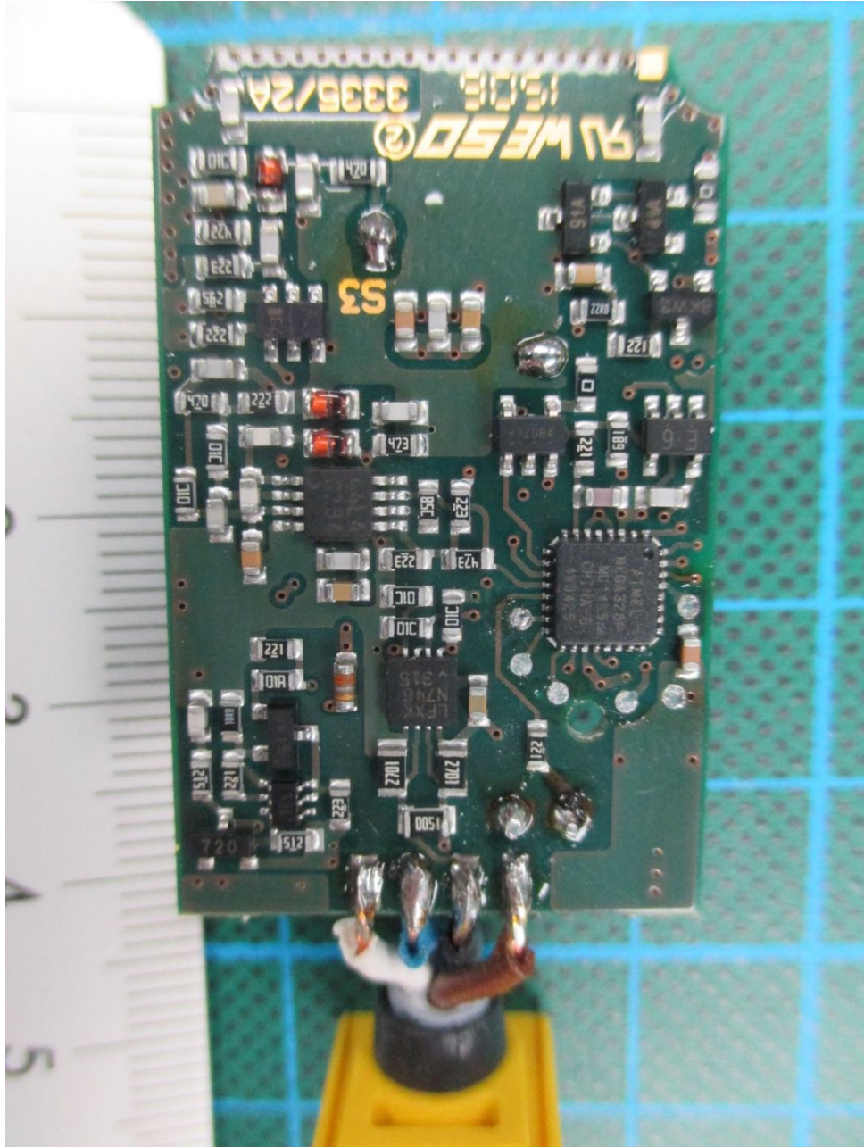
146168_12.JPG: TN-Q14-0.15-RS4.47T, PCB, rear view
