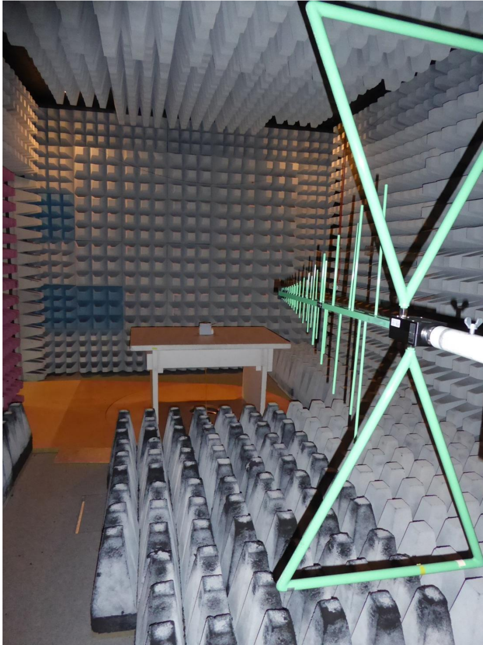
154999_2.JPG: Test setup fully anechoic chamber (E-Field)
