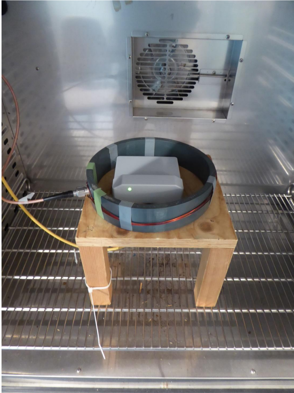
154999_6.JPG: Test setup temperature chamber
