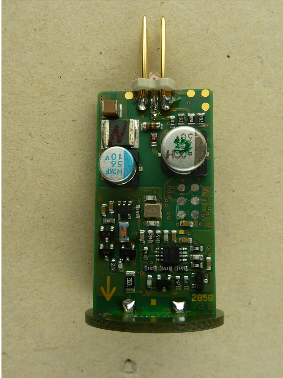
135060_12.JPG: TN-M30-H1147, PCB, top view
