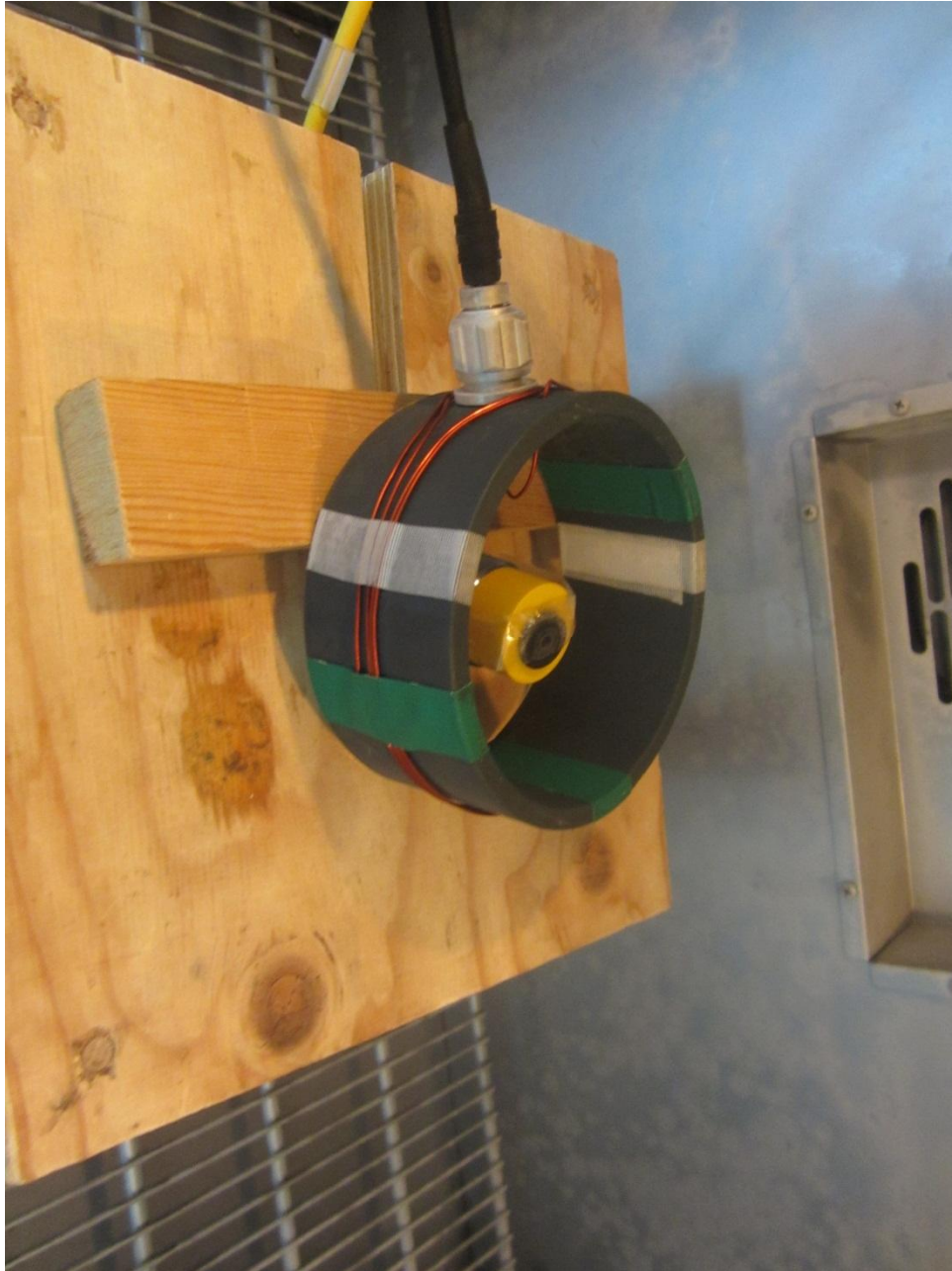
135060_6a.jpg: Test setup climatic chamber
