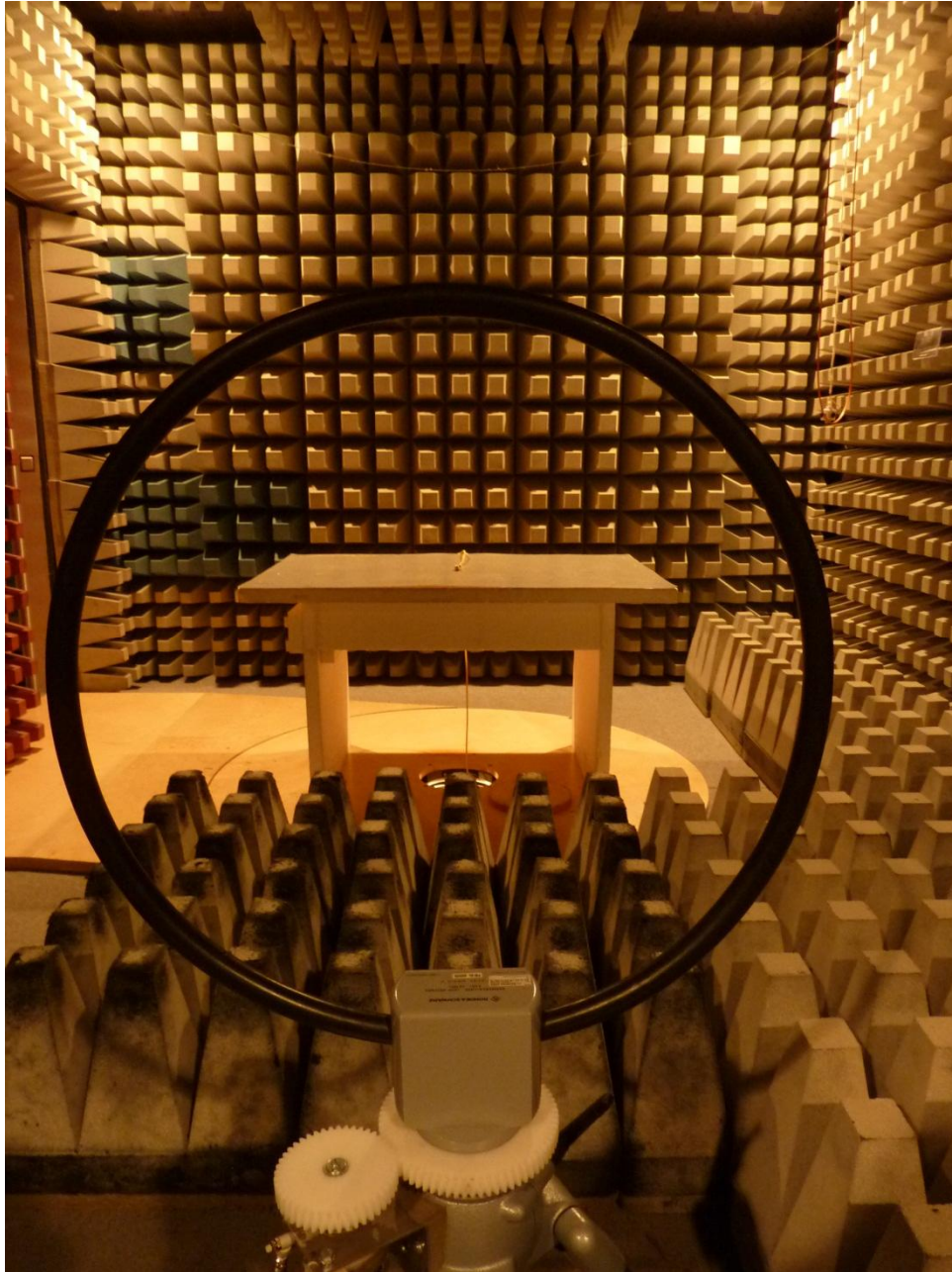
135060_3.JPG: Test setup fully anechoic chamber (H-Field)
