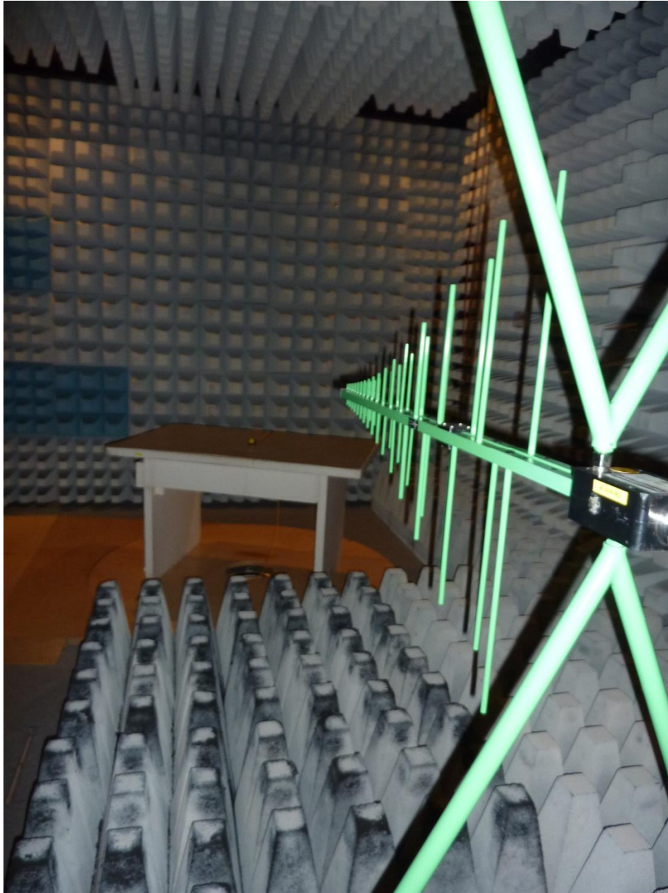
135060_2.JPG: Test setup fully anechoic chamber (E-Field)
