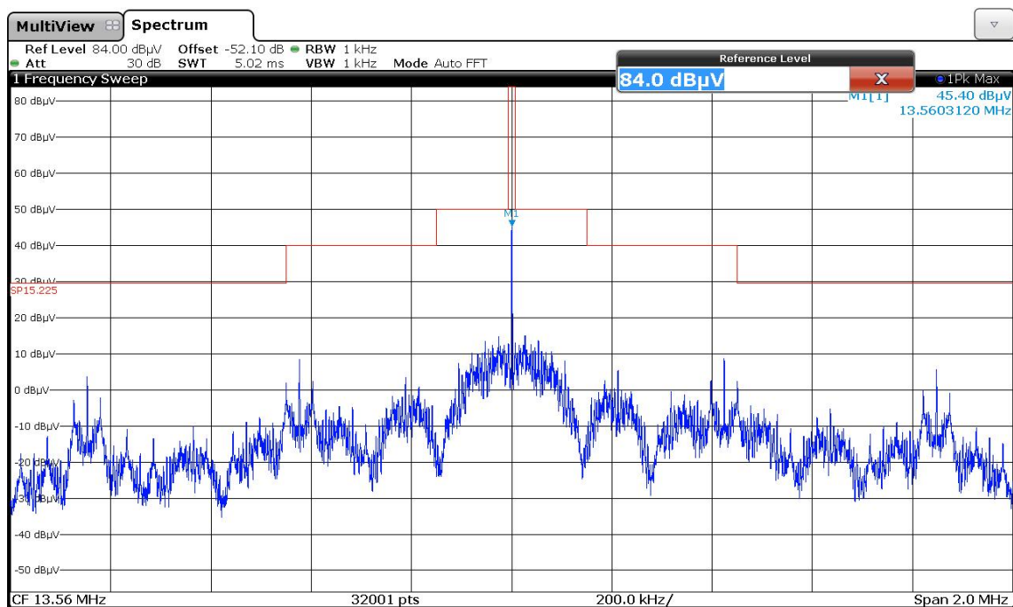
135060TNM30SM.png: Spectrum mask
