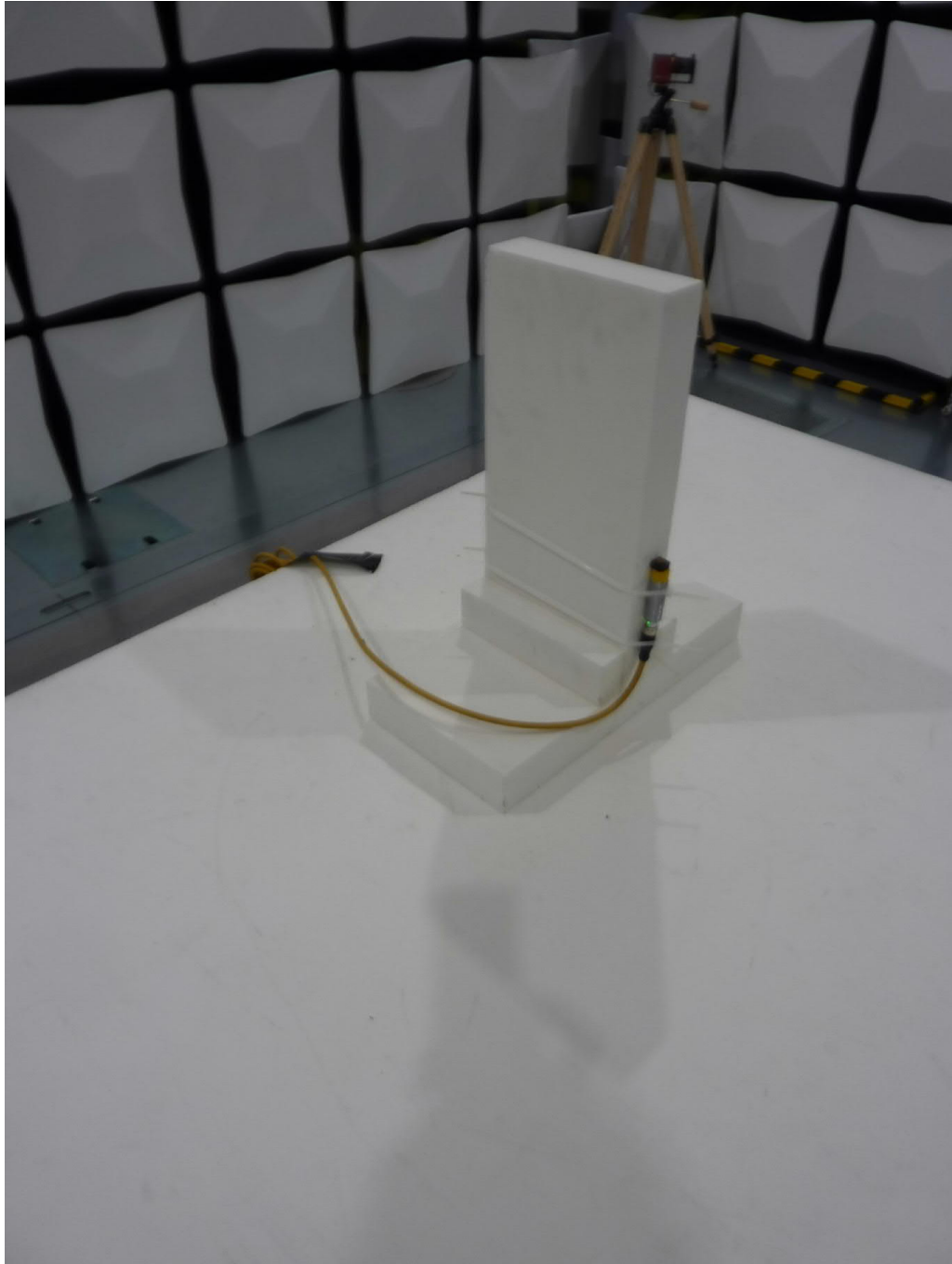
Test setup semi anechoic chamber (Pos. 2)
