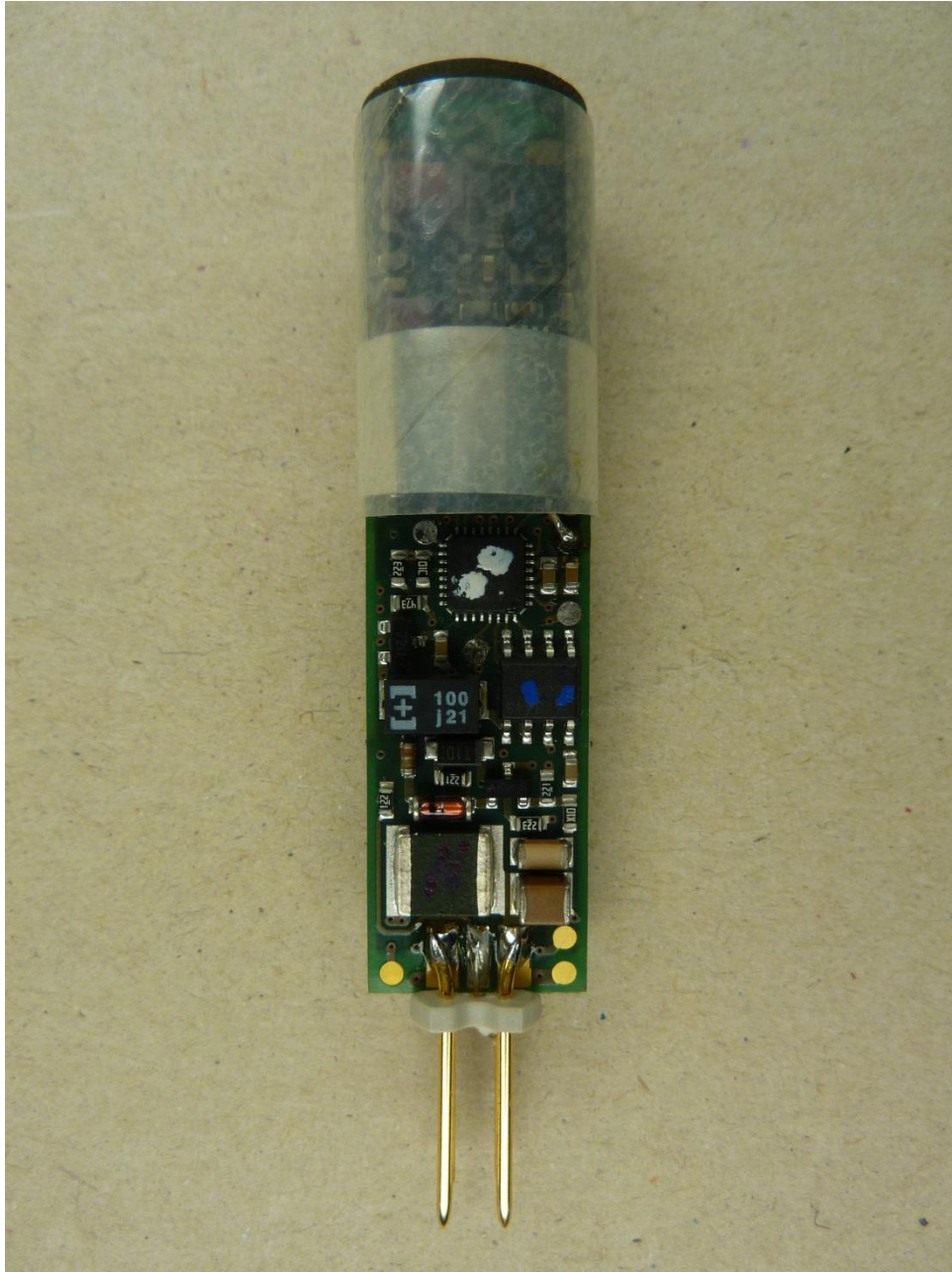
135074_10.JPG: TN-M18-H1147, PCB, top view
