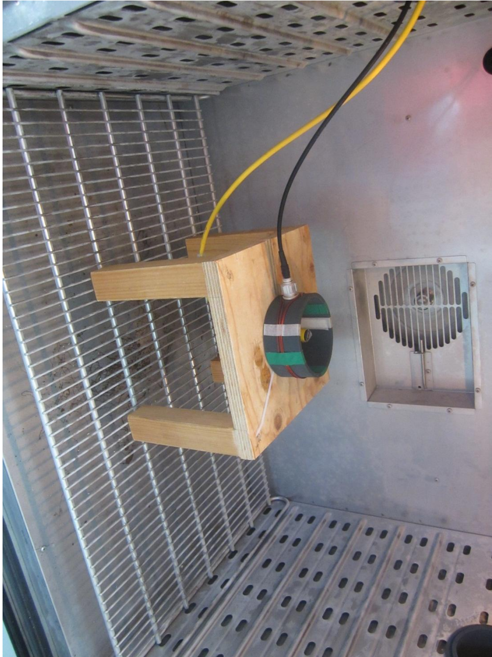
135074_22.JPG: Test setup climatic chamber
