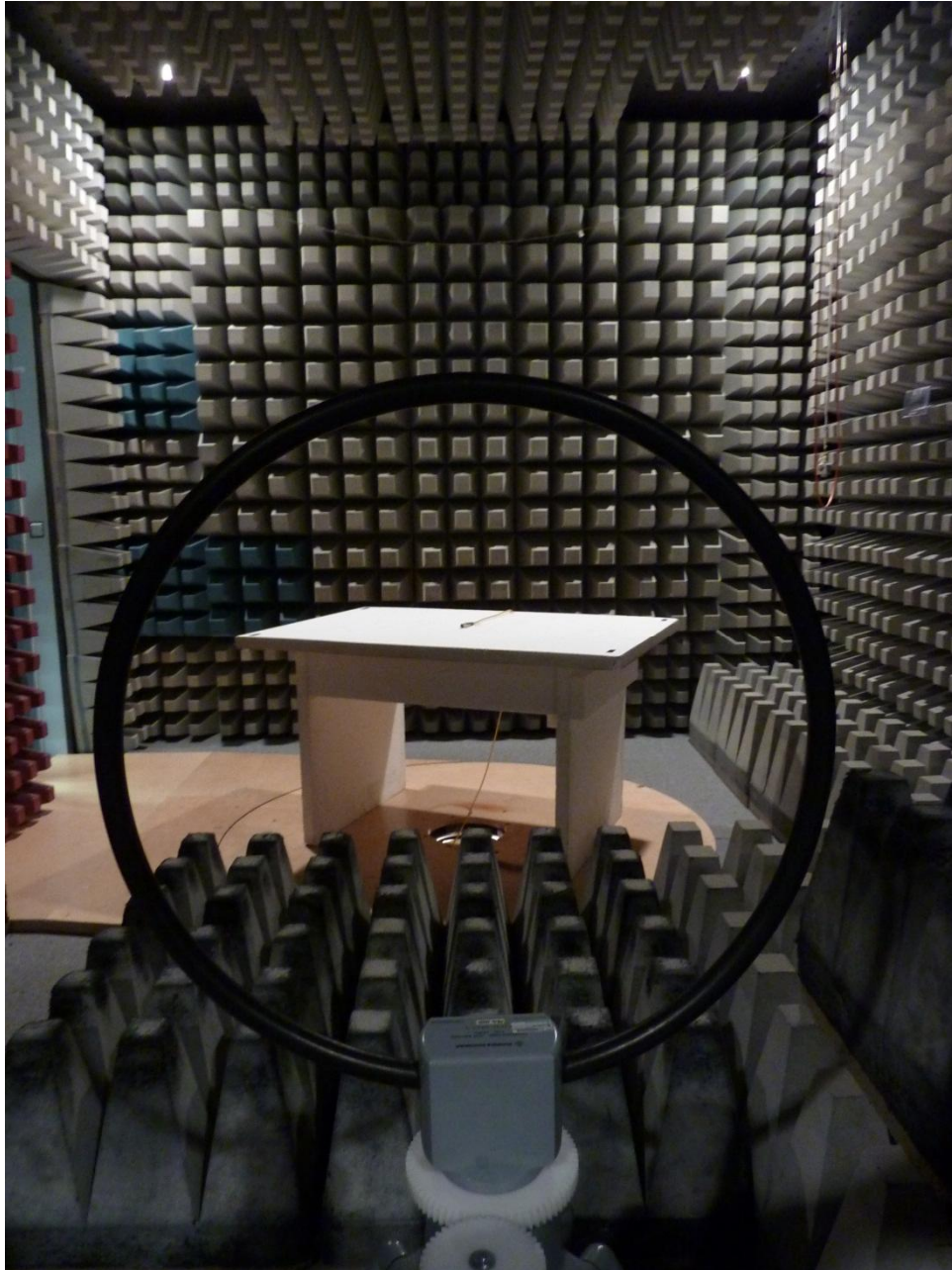
135074_19.JPG: Test setup fully anechoic chamber (H-Field)
