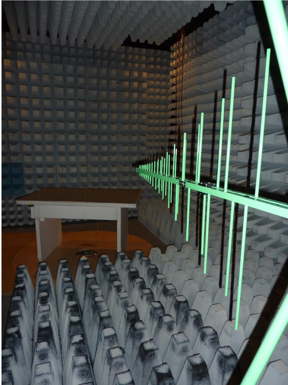
135074_18.JPG: Test setup fully anechoic chamber (E-Field)
