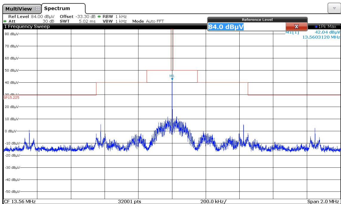
135074TNM18SM.png: Spectrum mask
