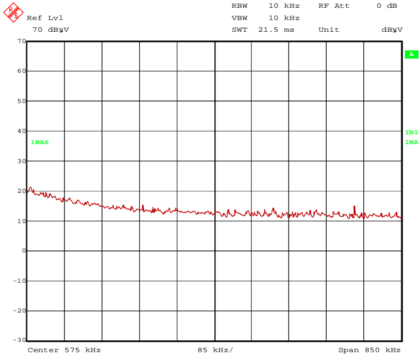
135074_b.wmf: Spurious emissions from 150 kHz to 1 MHz
