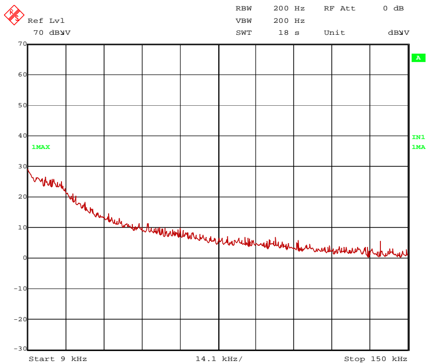
135074_a.wmf: Spurious emissions from 9 kHz to 150 kHz
