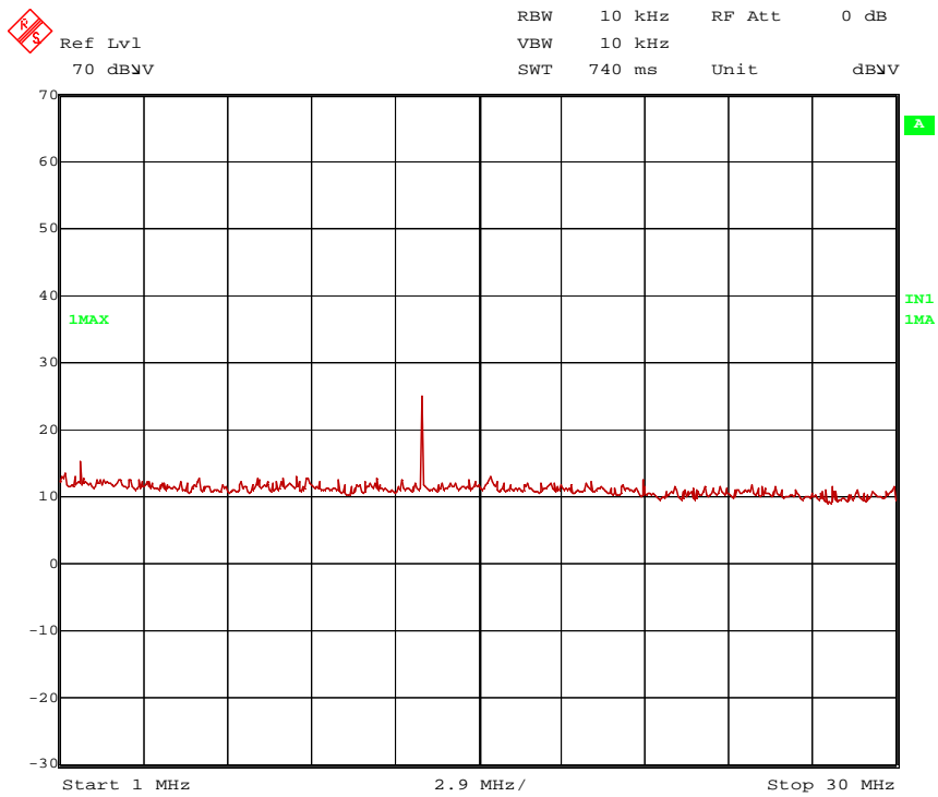
135074_c.wmf: Spurious emissions from 1 MHz to 30 MHz
