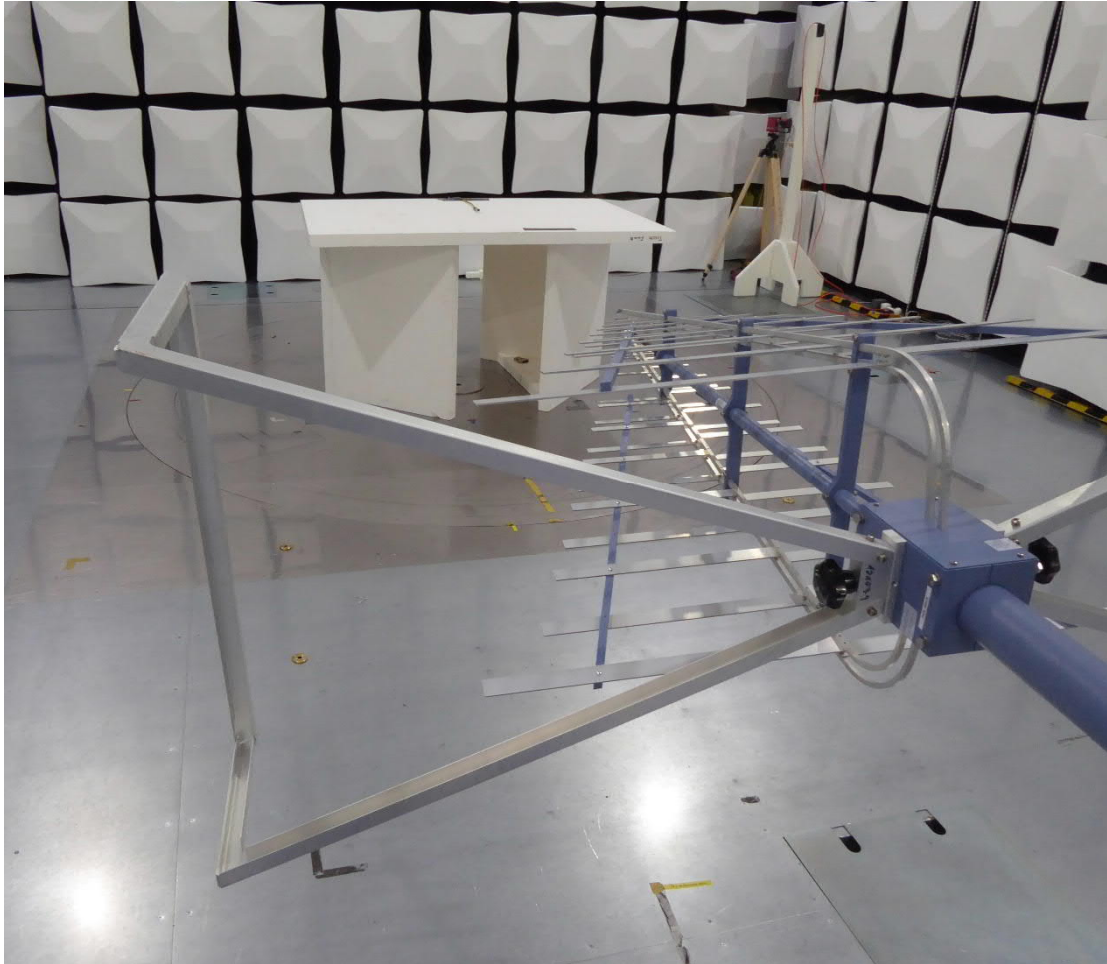
Test setup semi anechoic chamber (30 MHz to 1 GHz)
