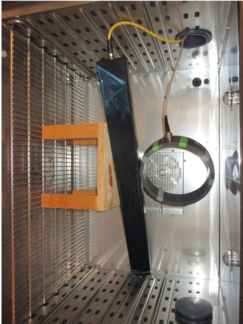
150253_6.JPG: Test setup temperature chamber
