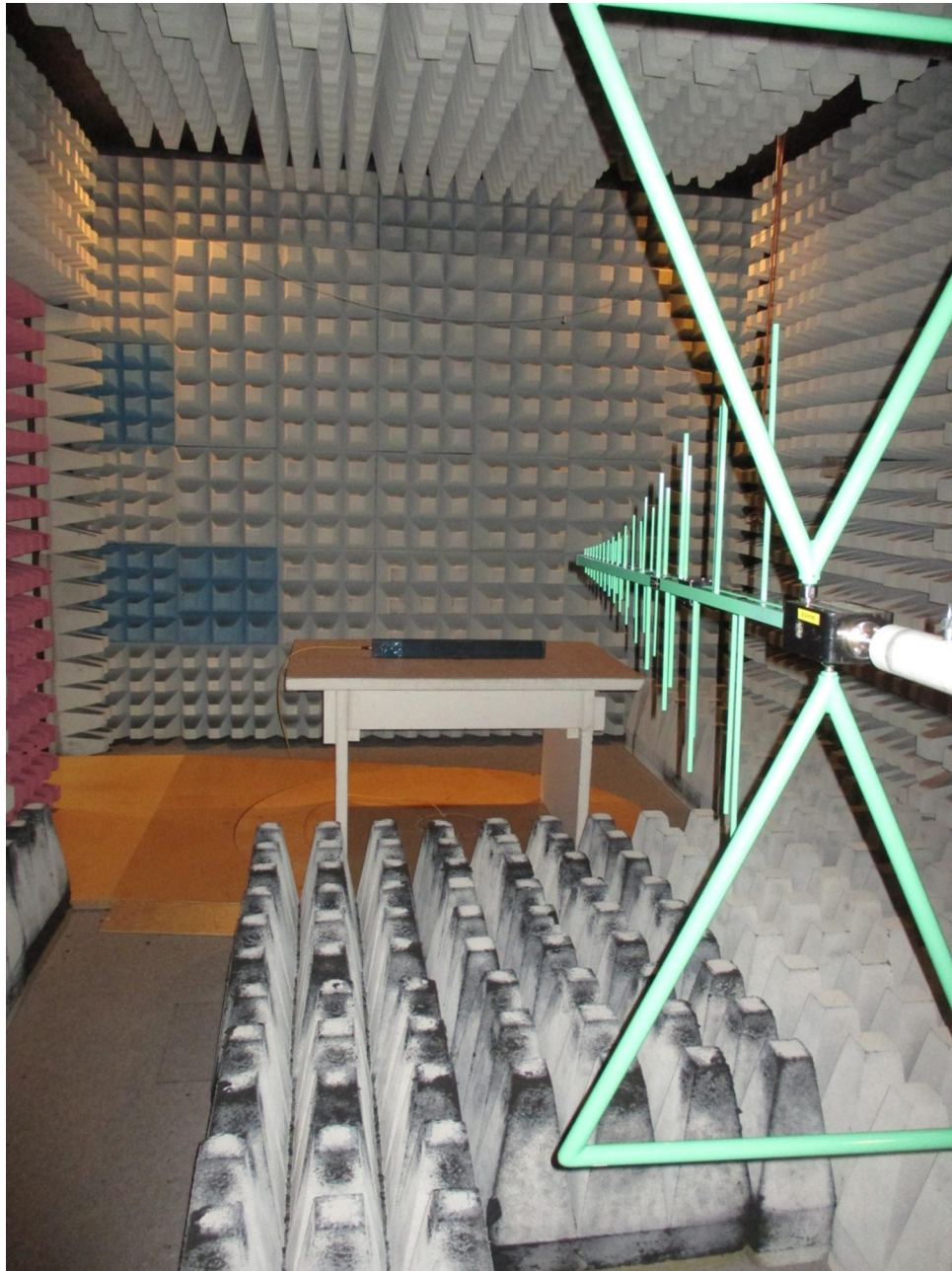
150253_2.JPG: Test setup fully anechoic chamber (E-Field)
