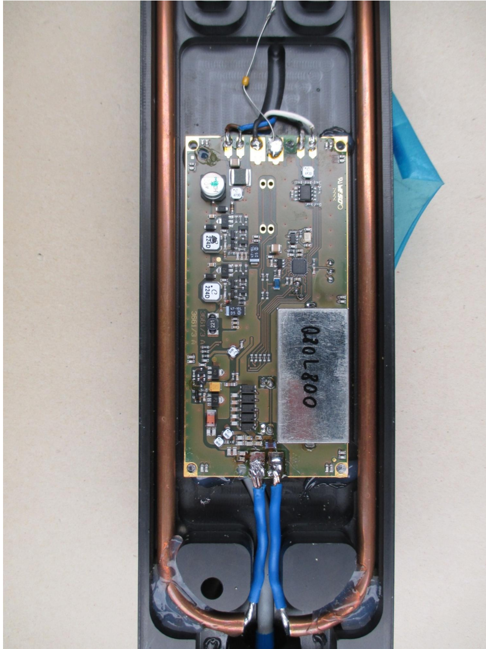
150253_11.JPG: TNLR-Q80L800-H1147, PCB, bottom view
