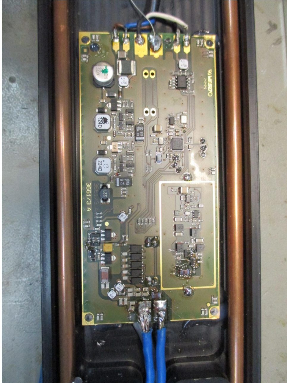
150253_12.JPG: TNLR-Q80L800-H1147, PCB, bottom view, shielding removed
