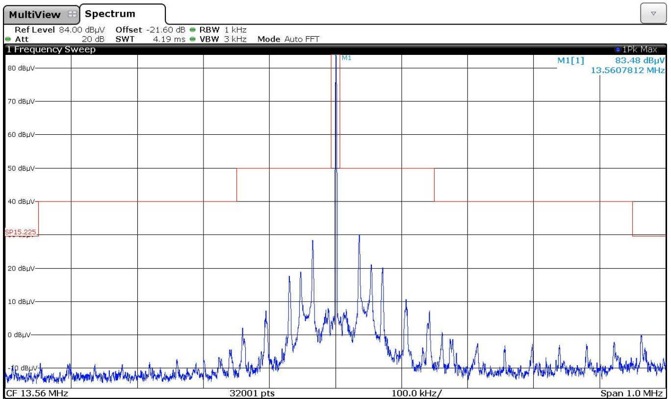
150253_20DEG_24V.wmf: Spectrum mask
