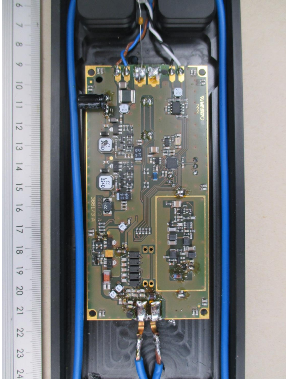
150254_12.JPG: TNLR-Q80L400-H1147, PCB, bottom view, shielding removed
