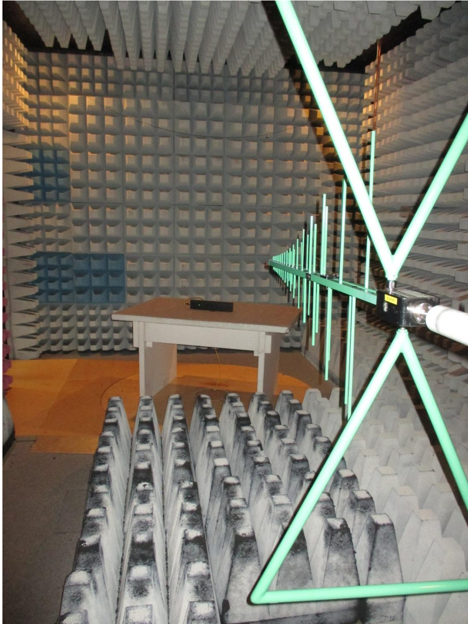
150254_2.JPG: Test setup fully anechoic chamber (E-Field)
