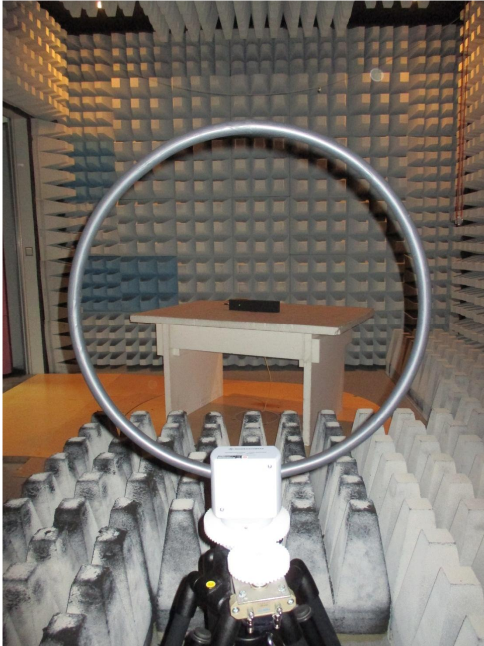
150254_3.JPG: Test setup fully anechoic chamber (H-Field)
