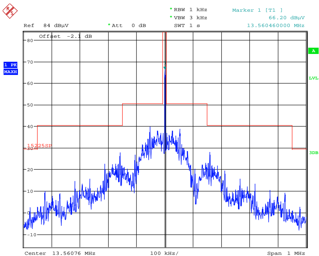
150254_20DEG_24V.wmf: Spectrum mask
