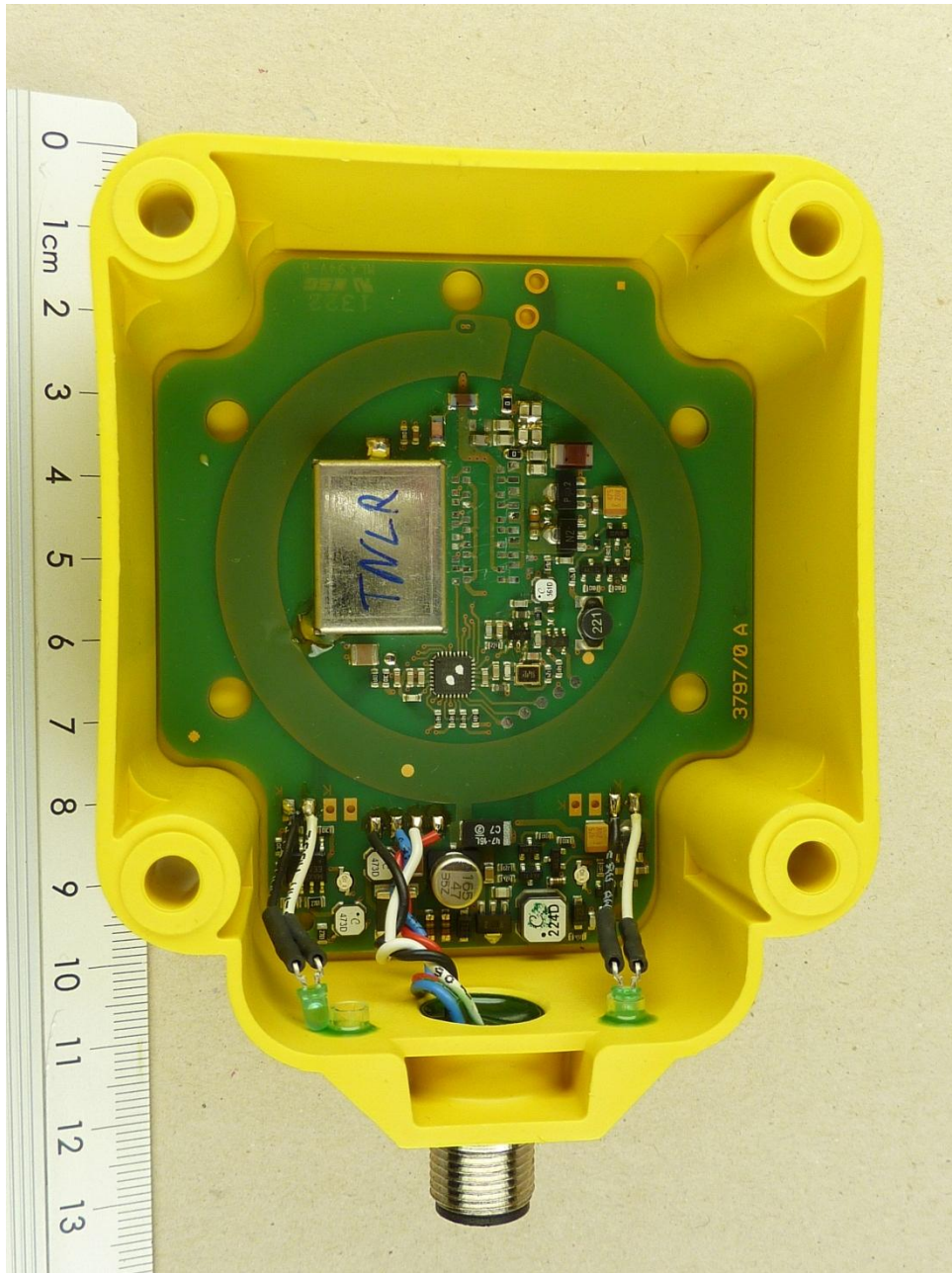
135058_8.JPG: TNLR-Q80-H1147, rear view to PCB
