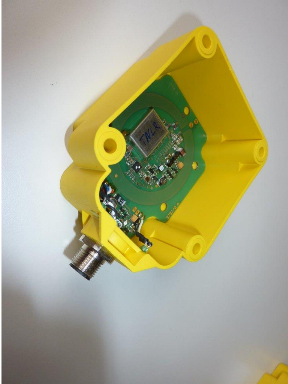
TNLR-Q80-3D2.JPG: TNLR-Q80-H1147, 3D view 2
