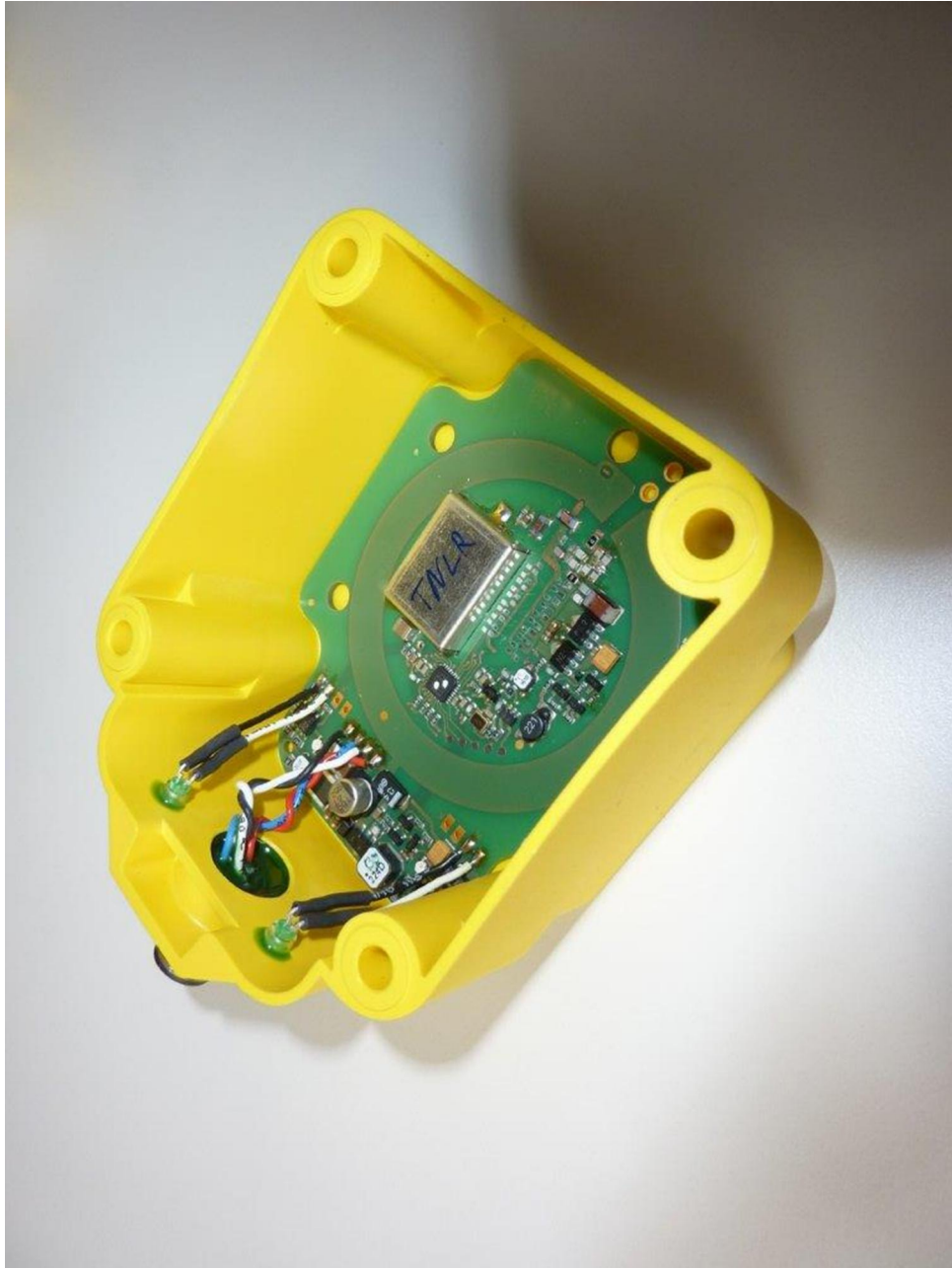
TNLR-Q80-3D1.JPG: TNLR-Q80-H1147, 3D view 1
