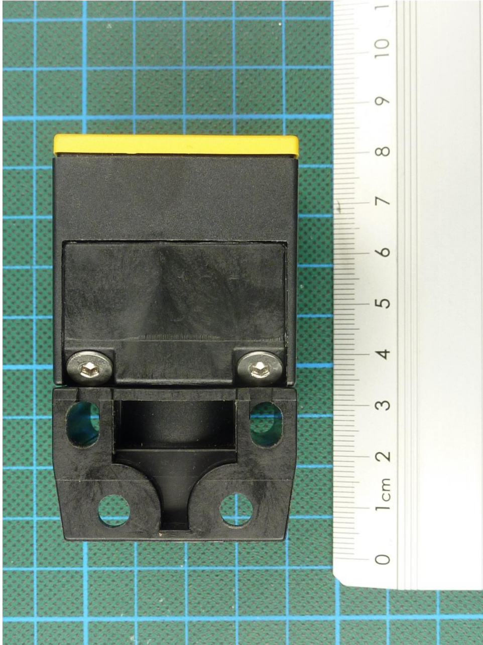
153588_8.JPG: TN-CK40-H1147, rear view
