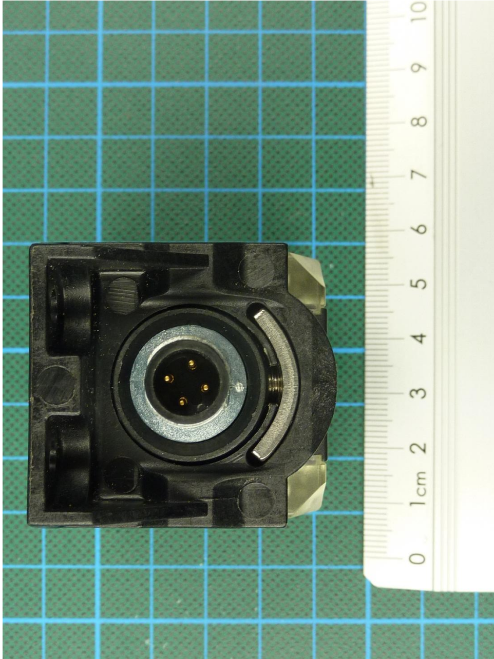
153588_10.JPG: TN-CK40-H1147, bottom view
