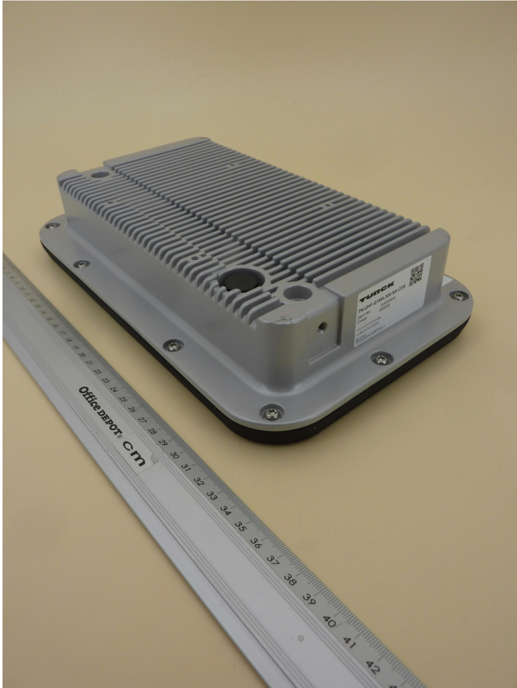
TN-UHF-Q180L300-NA-CDS, 3-D-view 2
