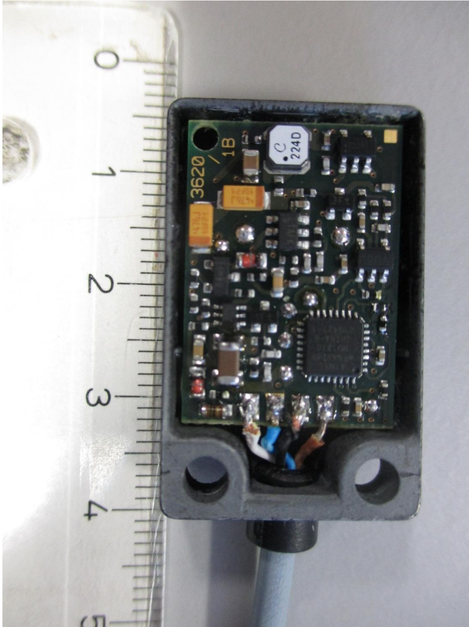
135053_7.JPG: TB-Q08-0.15-RS4.47T, bottom view (not grouted, PCB bottom visible)
