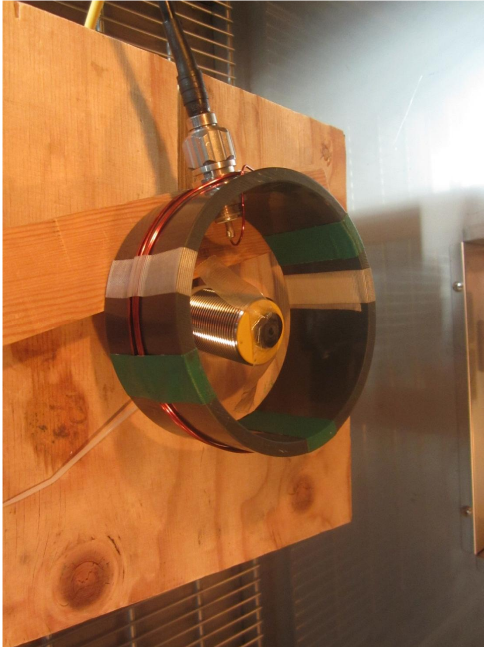
135060_6.jpg: Test setup climatic chamber
