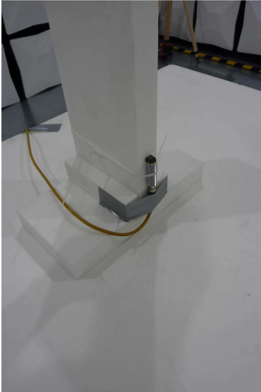
Test setup semi anechoic chamber (Pos. 2)
