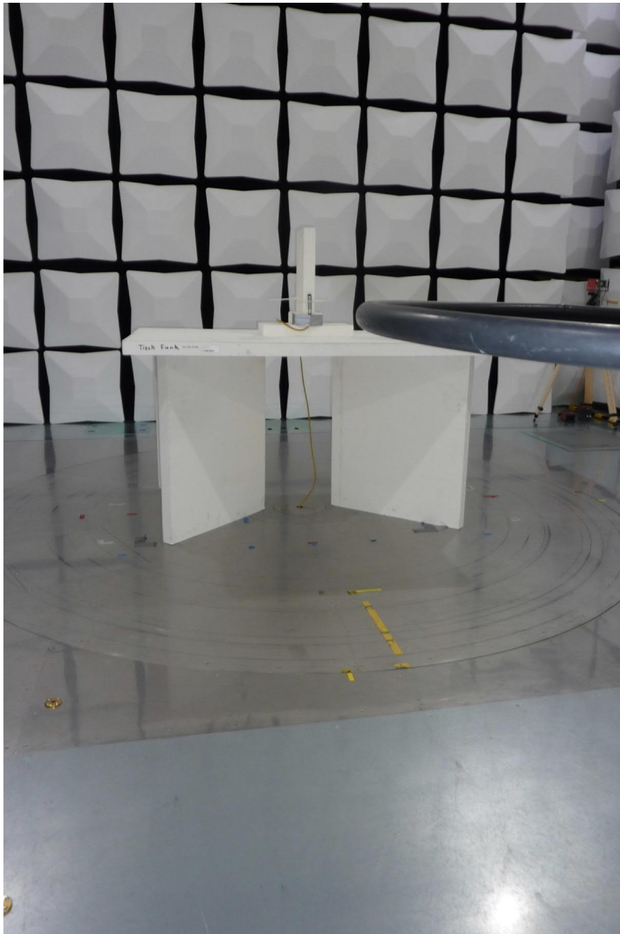
Test setup semi anechoic chamber (9 kHz to 30 MHz)
