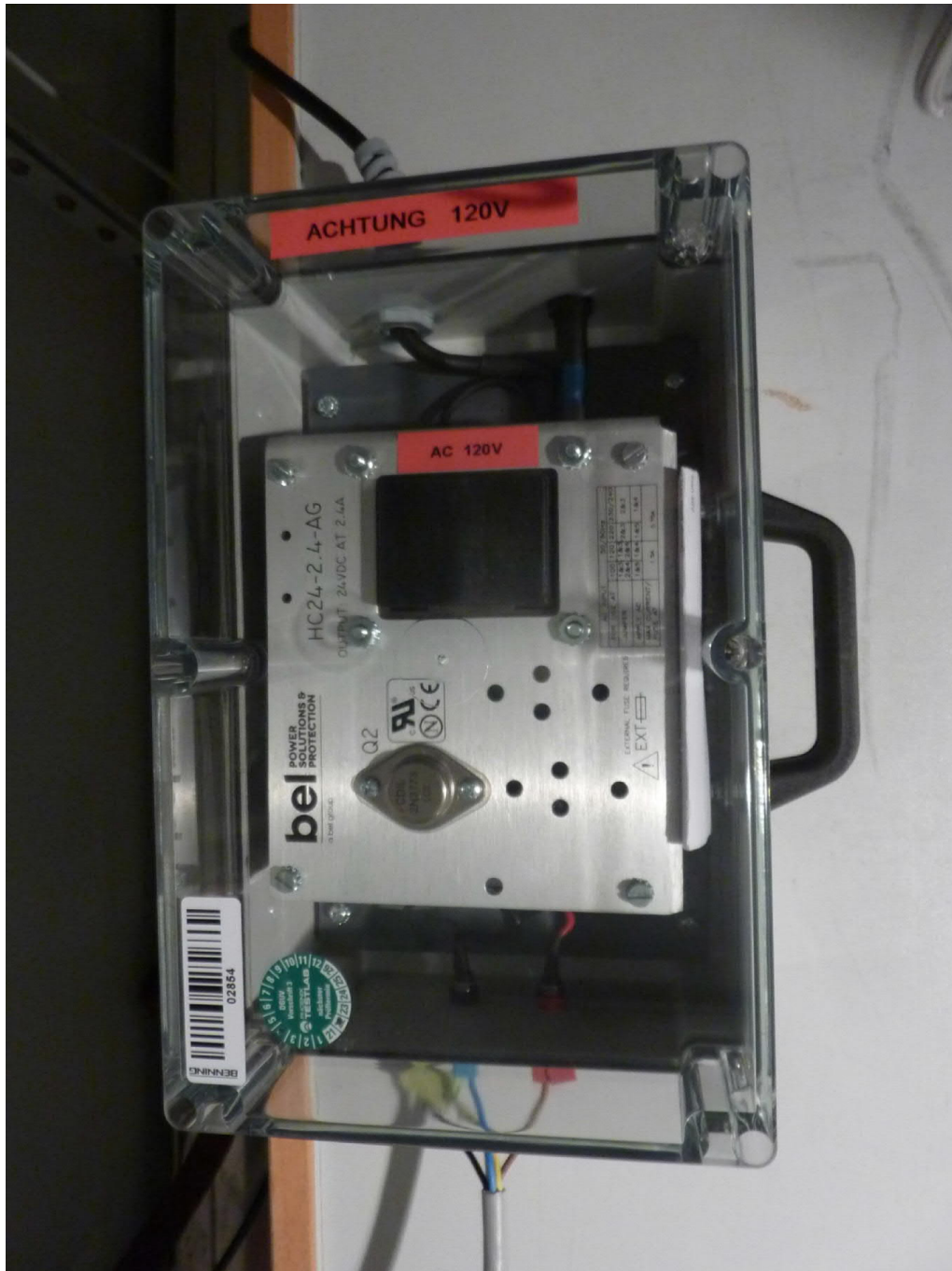
Power supply HC24-2.4 AG
