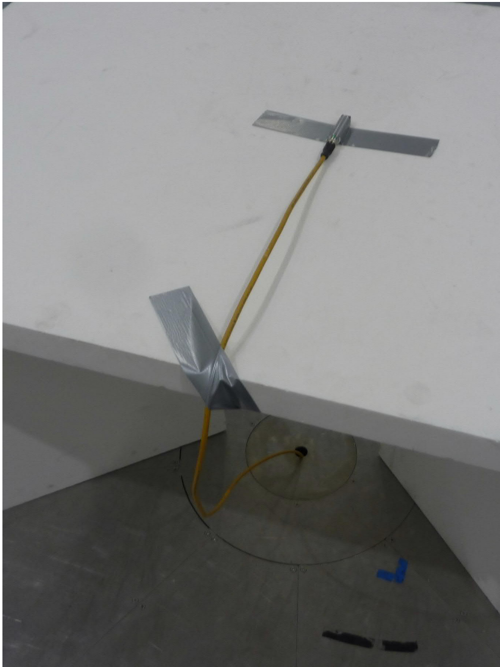
Test setup semi anechoic chamber (Pos. 1)
