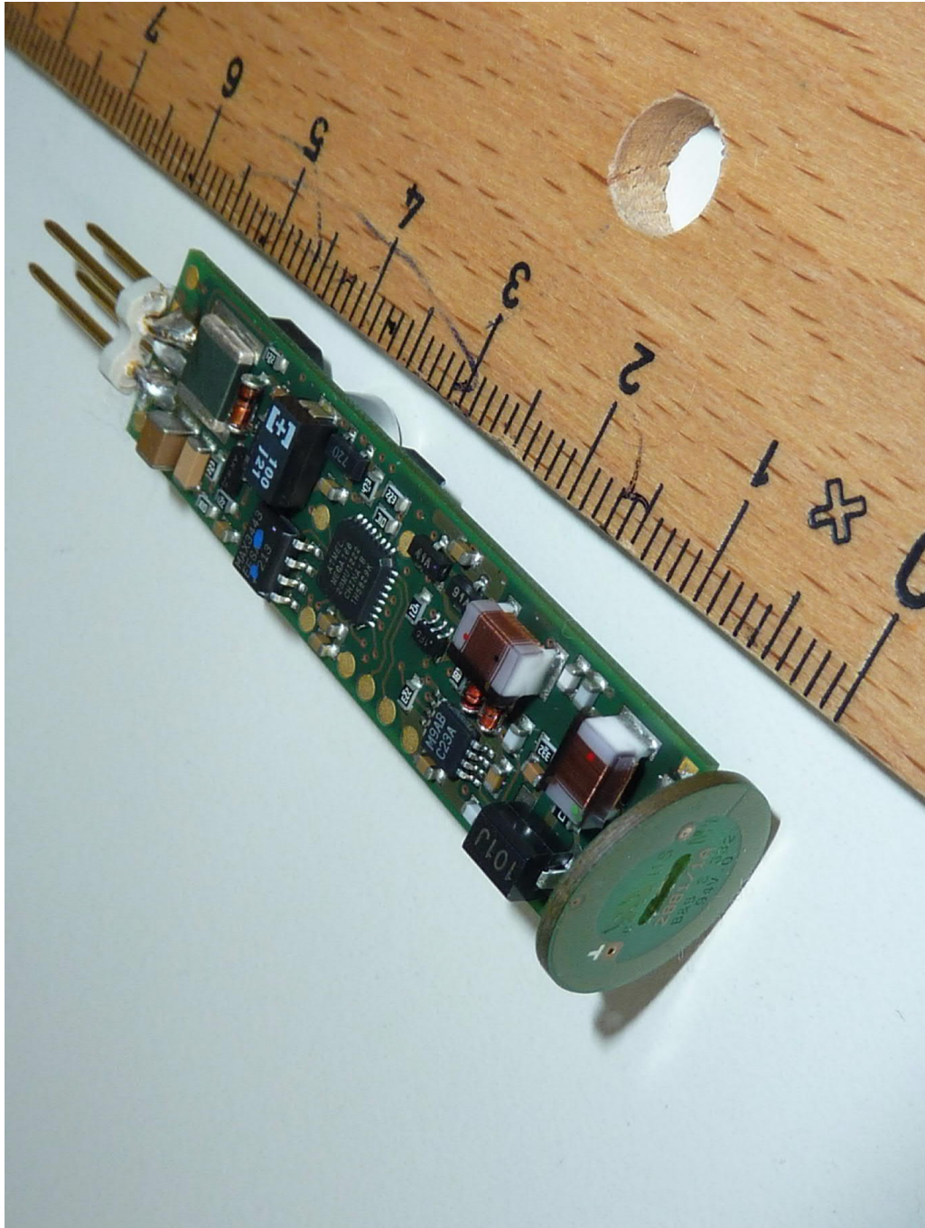
PCB, bottom view (photo provided by the applicant)
