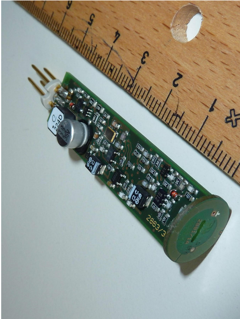
PCB, top view (photo provided by the applicant)
