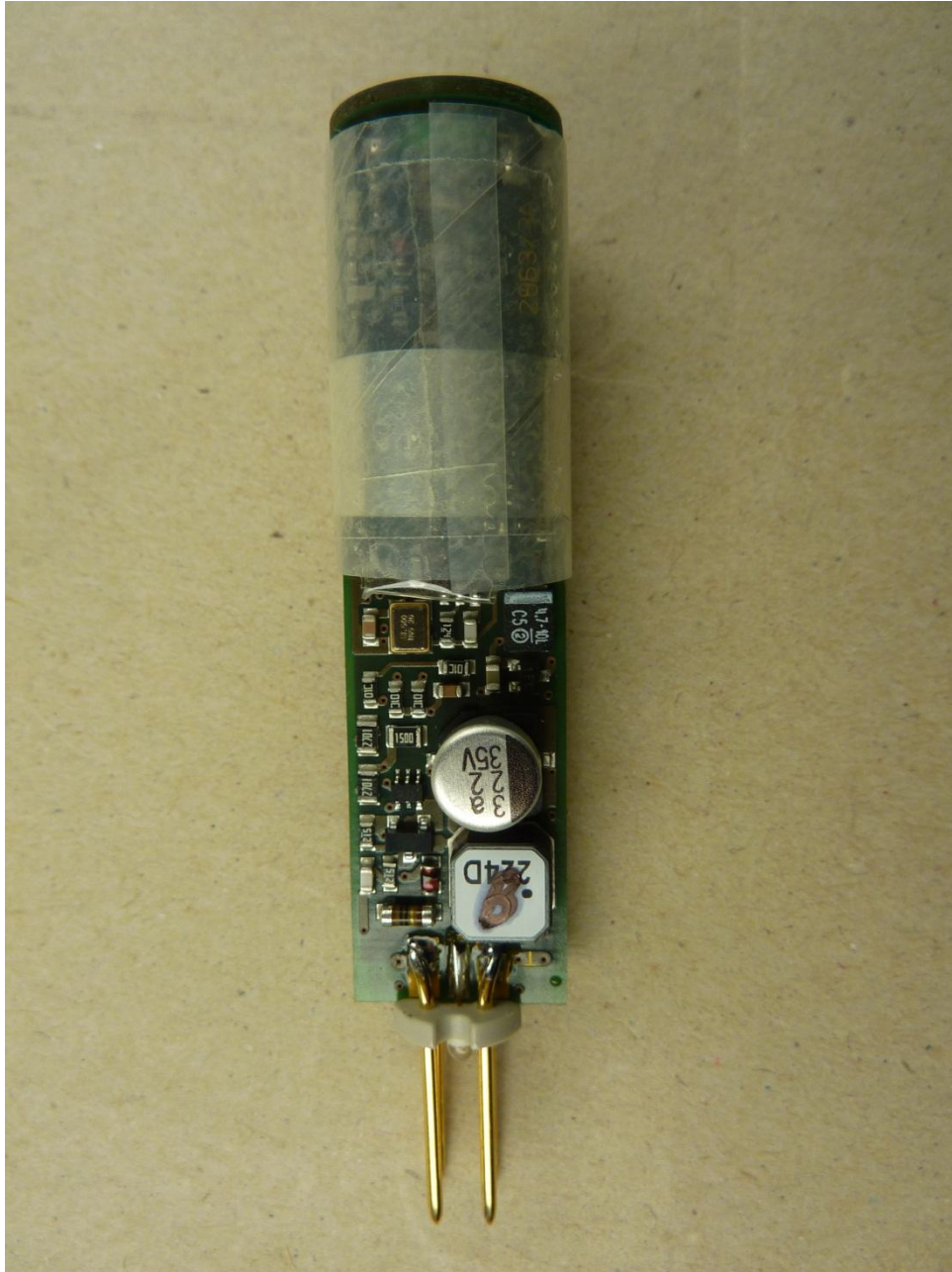
135074_14.JPG: TB-M18-H1147, PCB, bottom view
