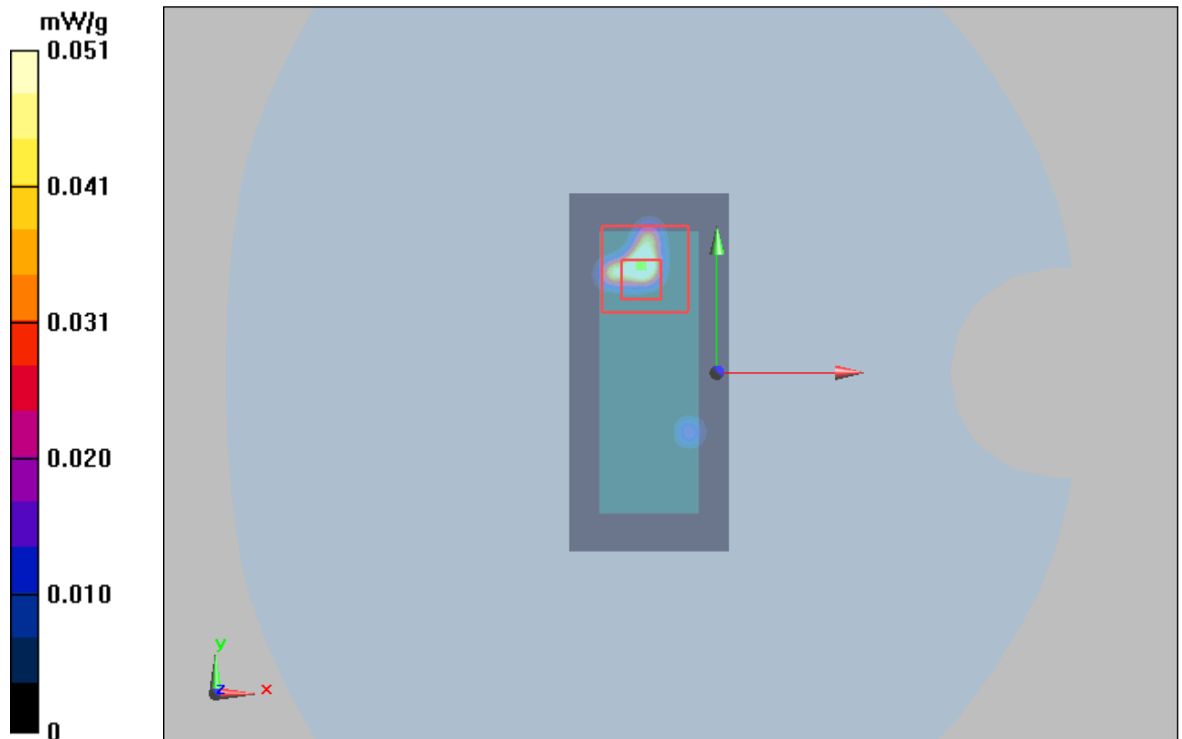
Figure 8 Test Position 2 5736MHz
