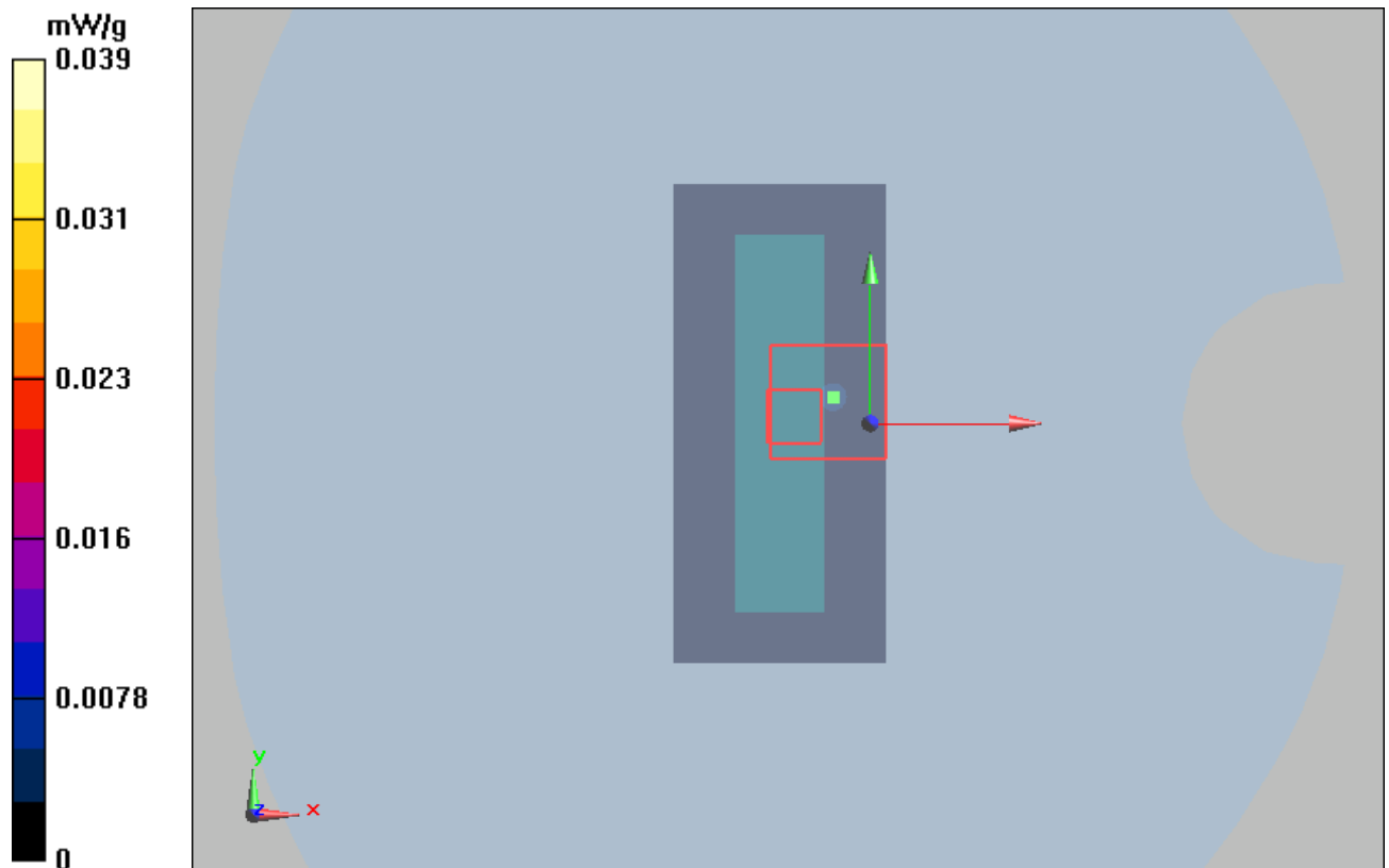
Figure 9 Test Position 3 5736MHz
