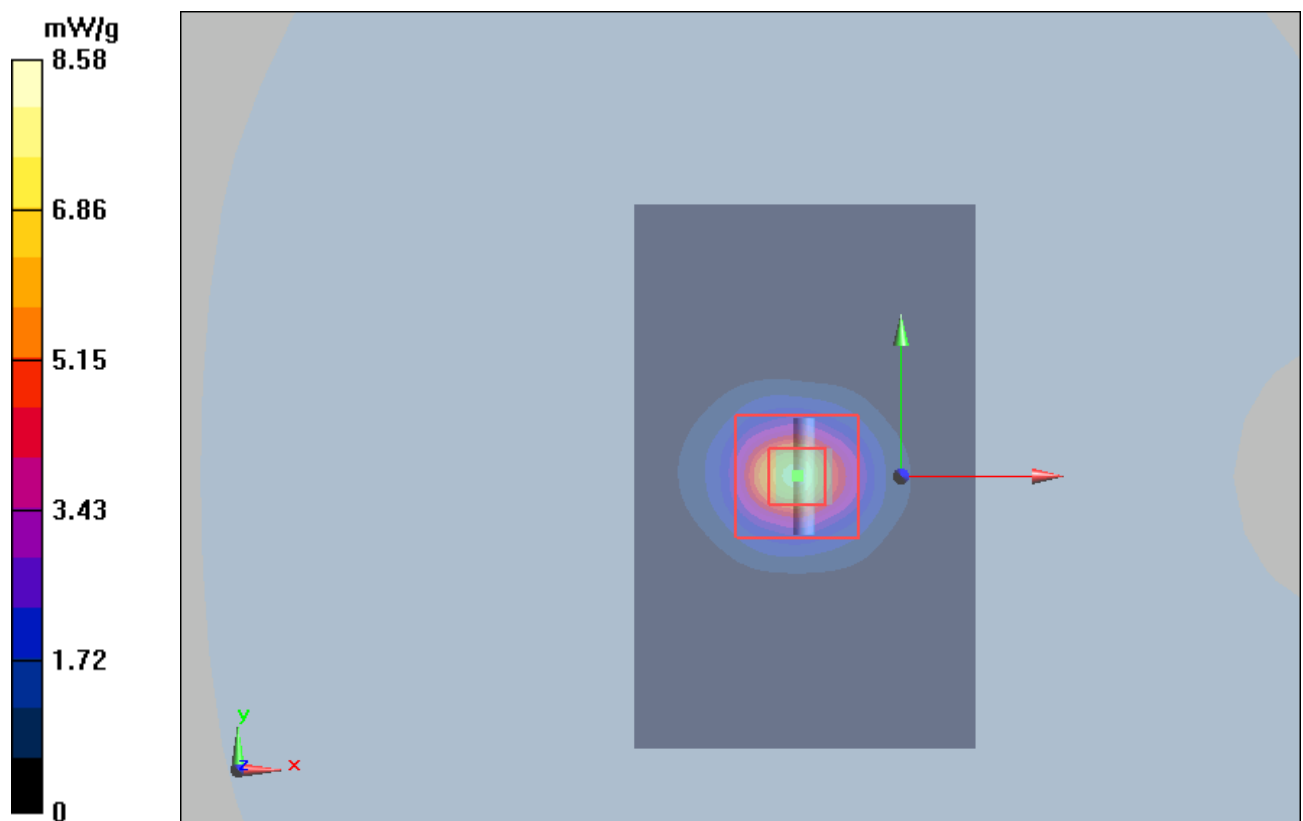
Figure 6 System Performance Check 5800MHz 100mW
