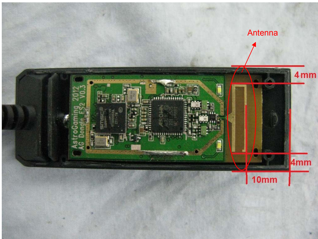
Picture 3: Constituents of the EUT
