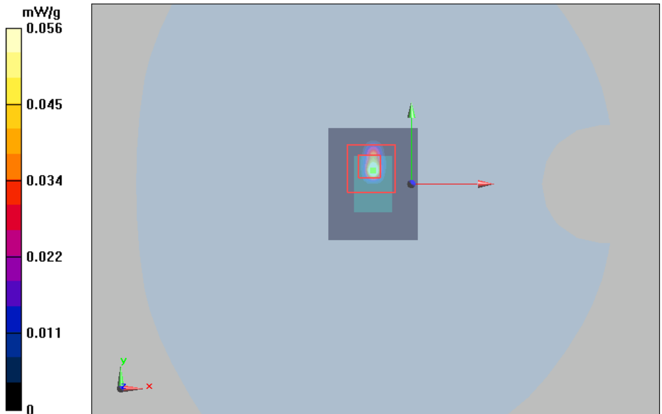
Figure 11 Test Position 5 5736MHz
