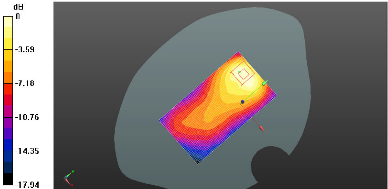
Plot 2: Body Rear Side (GSM850 GPRS 2TS Middle Channel)
