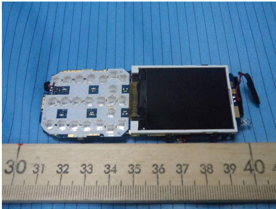
EUT – Main Board Bottom with LCD and Keyboard View
