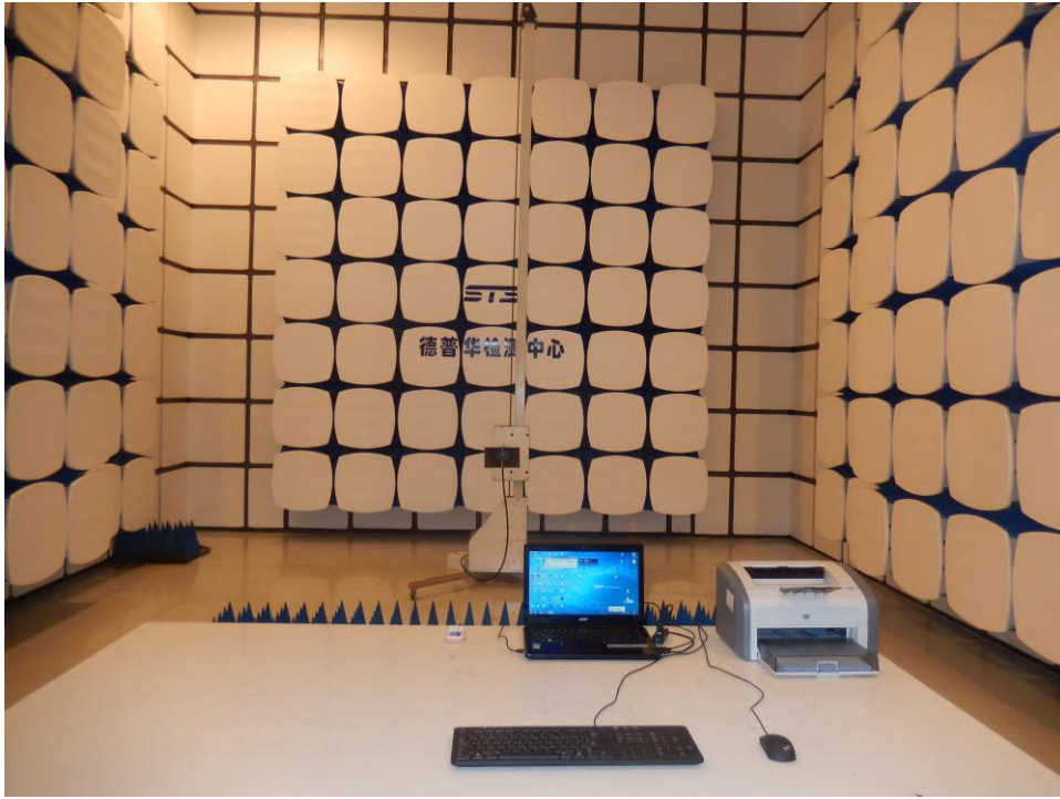
JBP radiation H
