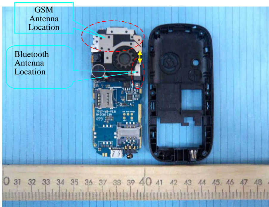
BT and GSM Antenna Location
