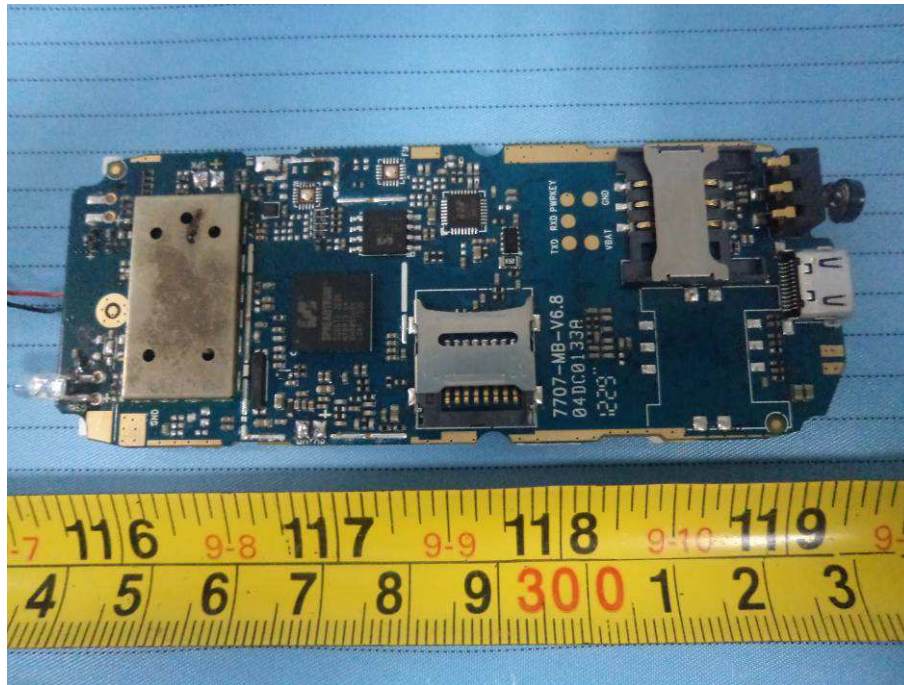
EUT – Main Board Bottom without GSM Antenna View
