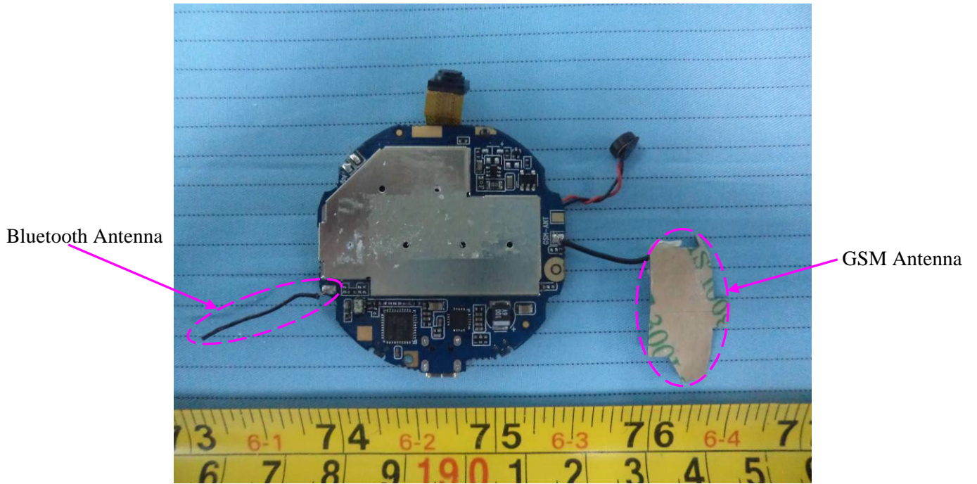
EUT – Main Board Bottom View
