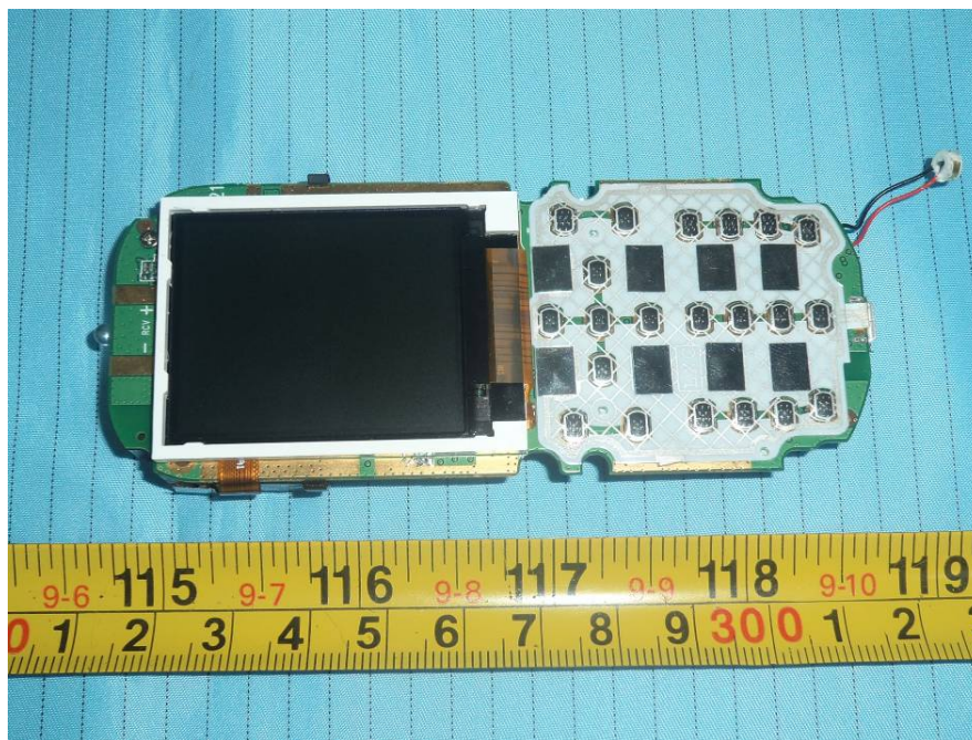
EUT – Main Board Bottom with LCD and Keyboard View
