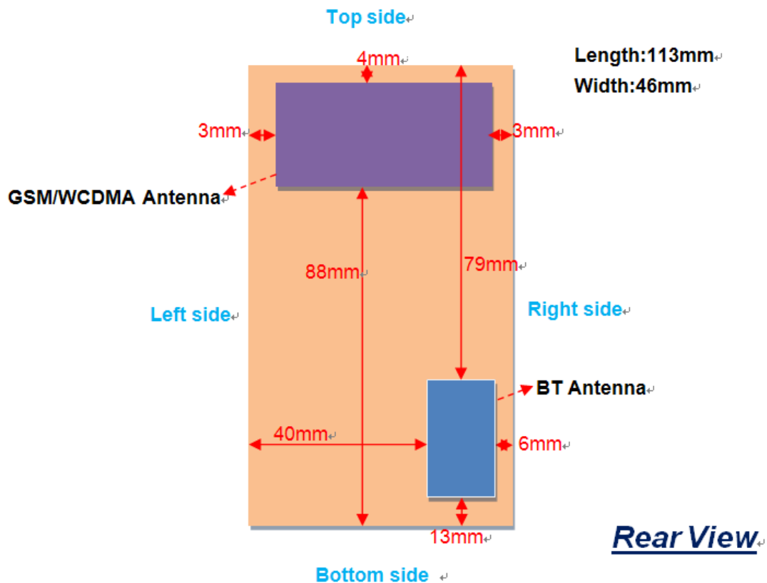
Figure 1: The antenna positions of the DUT
