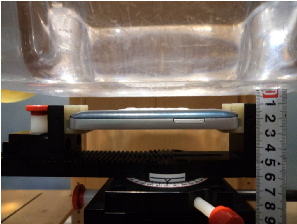
Body-worn Front Position D Setup Photo
