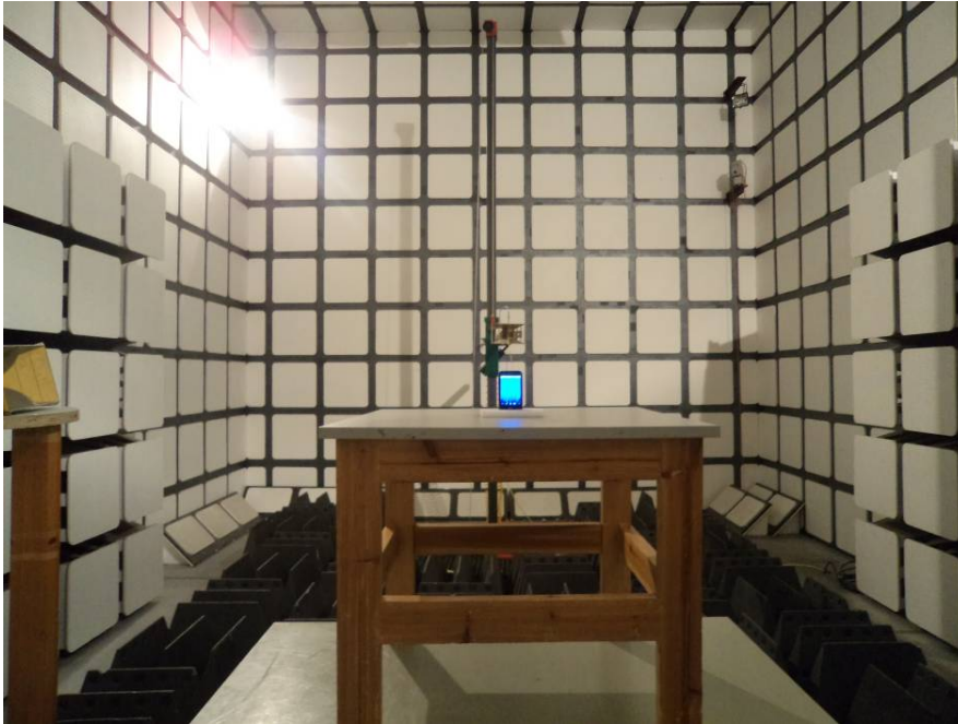
Radiated Emissions Test View
