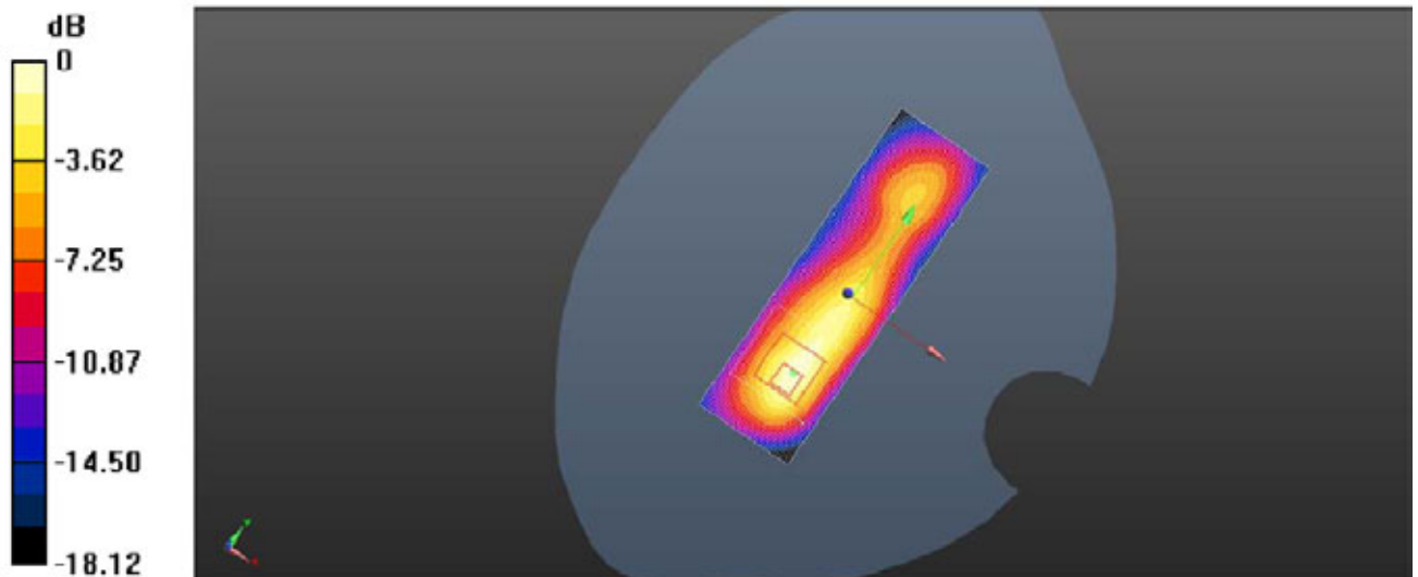
Plot 39: Body Left Side (WCDMA Band II RMC Middle Channel)
