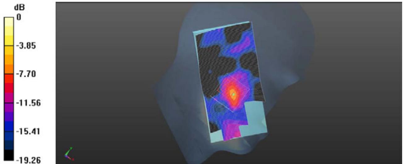
Plot 1: Left Head Touch (GSM850 Middle Channel)
