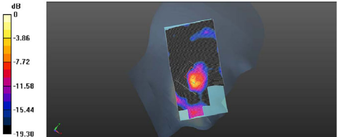
Plot 12: Left Head Touch (GSM1900 Middle Channel)
